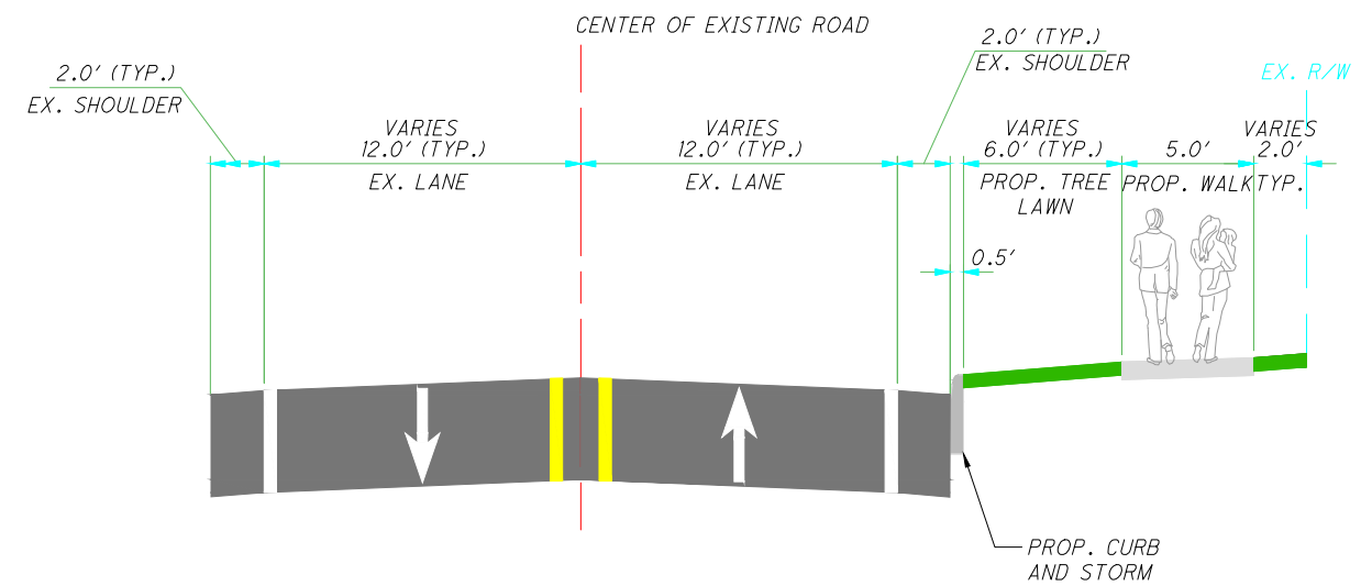
VALLEY VIEW ROAD - HUNTING HOLLOW DRIVE TO HINES HILL ROAD HINES HILL ROAD - VALLEY VIEW ROAD TO GLASTONBURY DRIVE (SHOWN PER DIRECTION OF TRAVEL, REVERSE AS NECESSARY) CURB SECTION - TREE LAWN
