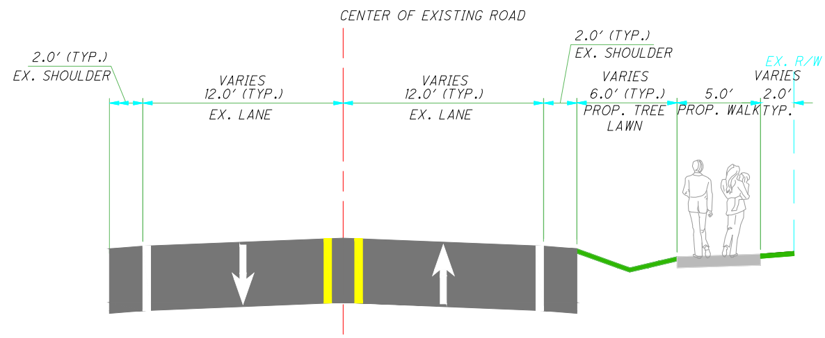
PREFERRED TYPICAL SECTION VALLEY VIEW ROAD - HUNTING HOLLOW DRIVE TO HINES HILL ROAD HINES HILL ROAD - VALLEY VIEW ROAD TO GLASTONBURY DRIVE (SHOWN PER DIRECTION OF TRAVEL, REVERSE AS NECESSARY) SWALE SECTION
