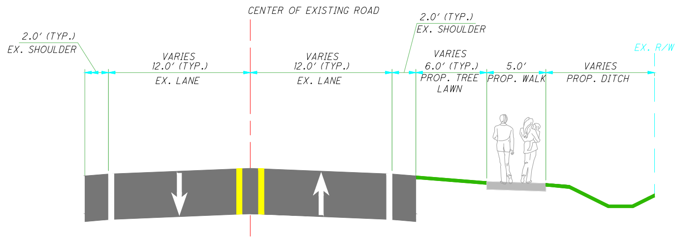
VALLEY VIEW ROAD - HUNTING HOLLOW DRIVE TO HINES HILL ROAD HINES HILL ROAD - VALLEY VIEW ROAD TO GLASTONBURY DRIVE (SHOWN PER DIRECTION OF TRAVEL, REVERSE AS NECESSARY) DITCH SECTION
