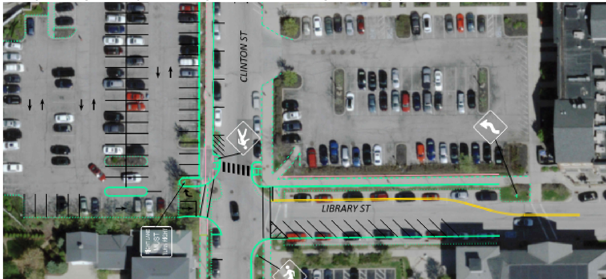
ALT 3 - REALIGNMENT OF LIBRARY STREET WITH EX. WEST ENTRANCE/EXIT
