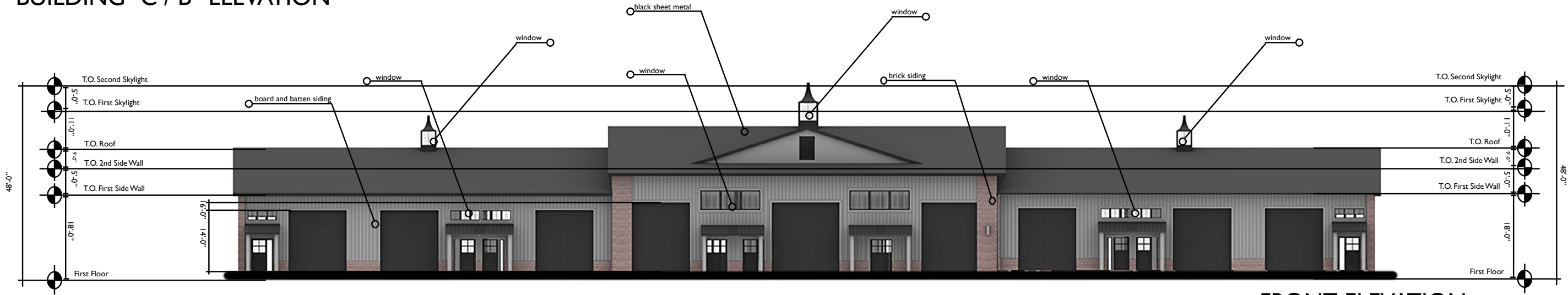
FRONT ELEVATION
