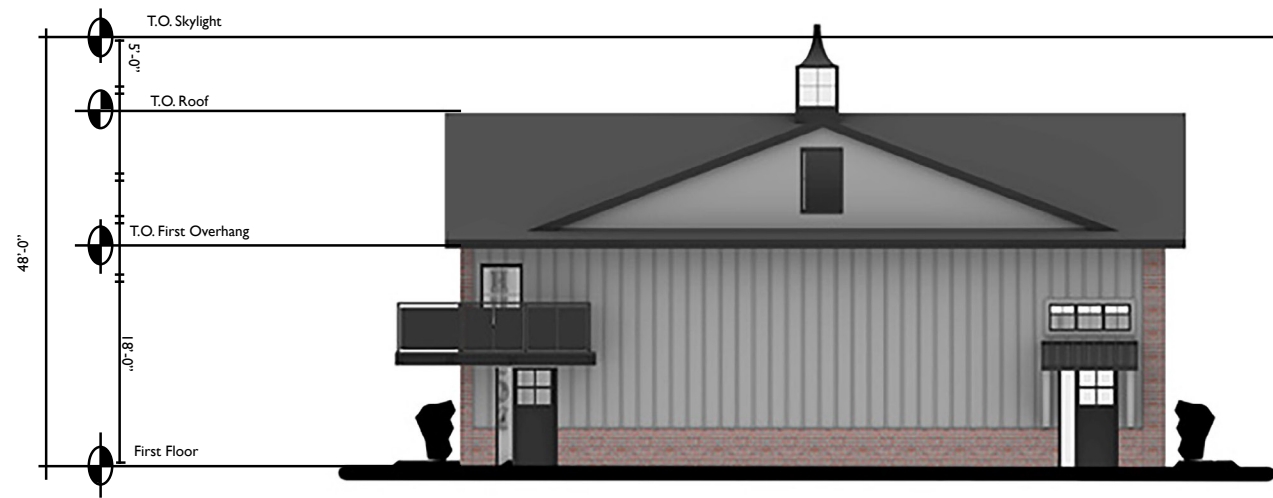
REAR ELEVATION
