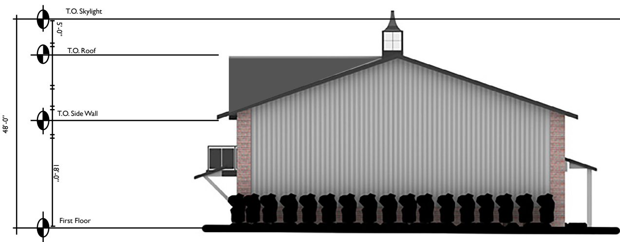
SIDE ELEVATION
