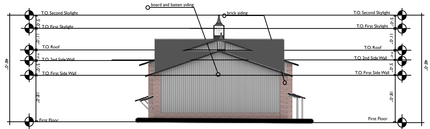
SIDE ELEVATION
