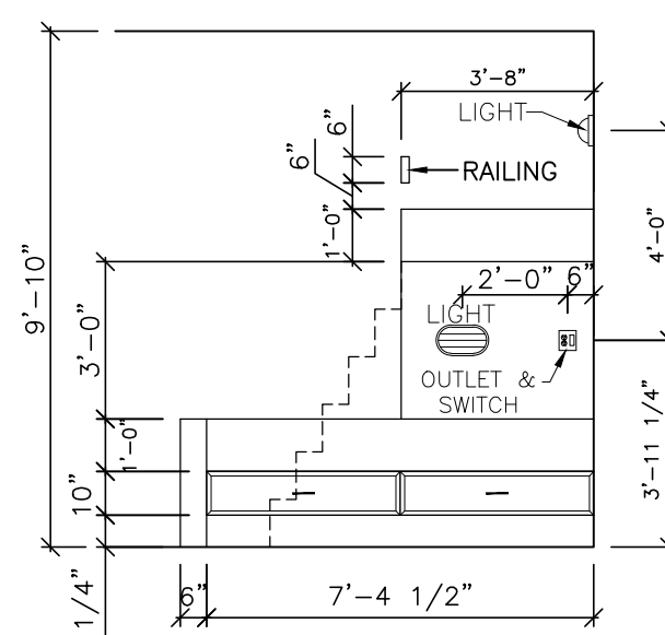
SIDE ELEVATION VIEW OF BUNK BED IN LOWER LEVEL SCALE: 1/4" = 1'-0"
