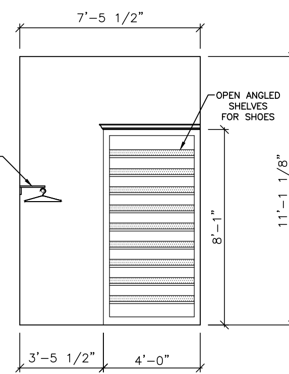
DETAIL OF WIC SHOE SHELVES SCALE: 1/4" = 1'-0"
