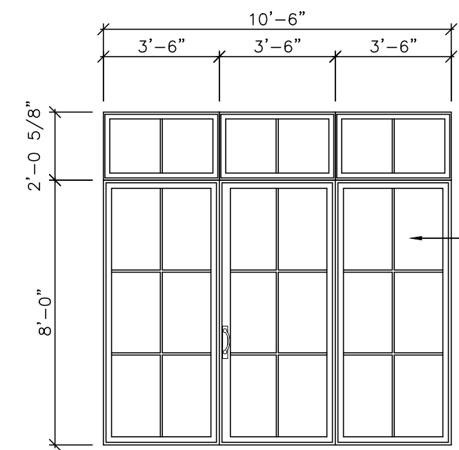
DETAIL OF DINING AREA DOOR AND TRANSOMS SCALE: 1/4" = 1'-0"
