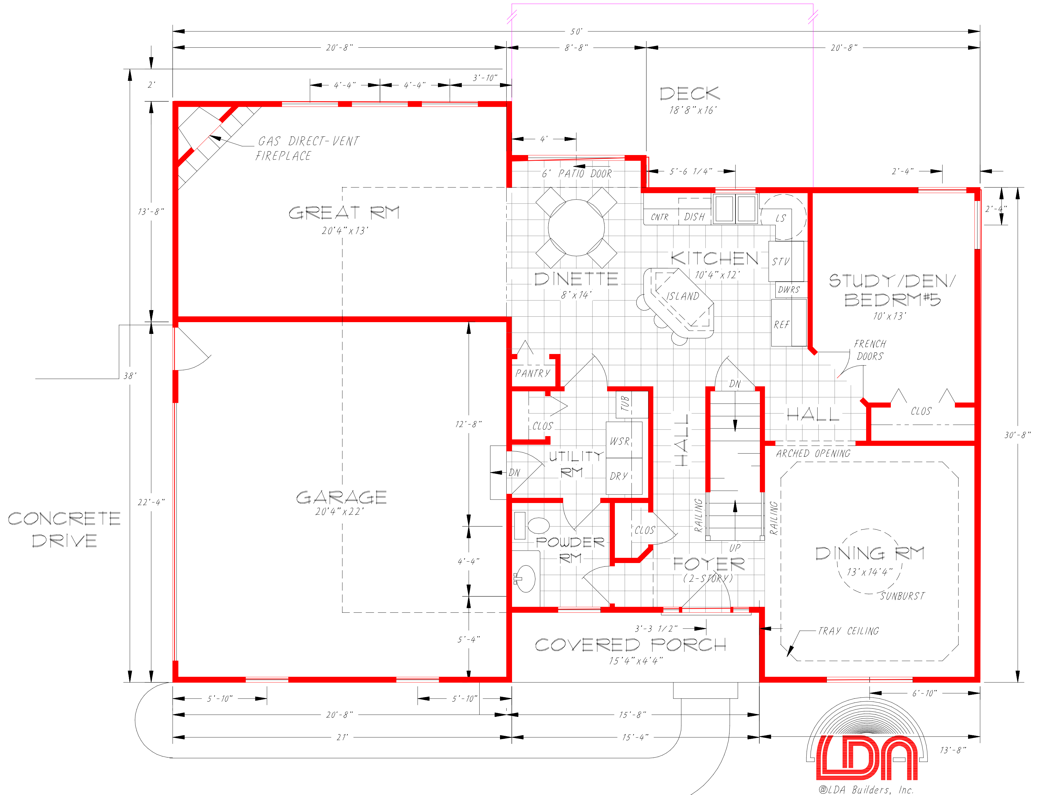
The Soulsby Residence "Riverwine" modified 2182 sq.ft. 1st Floor 090118
