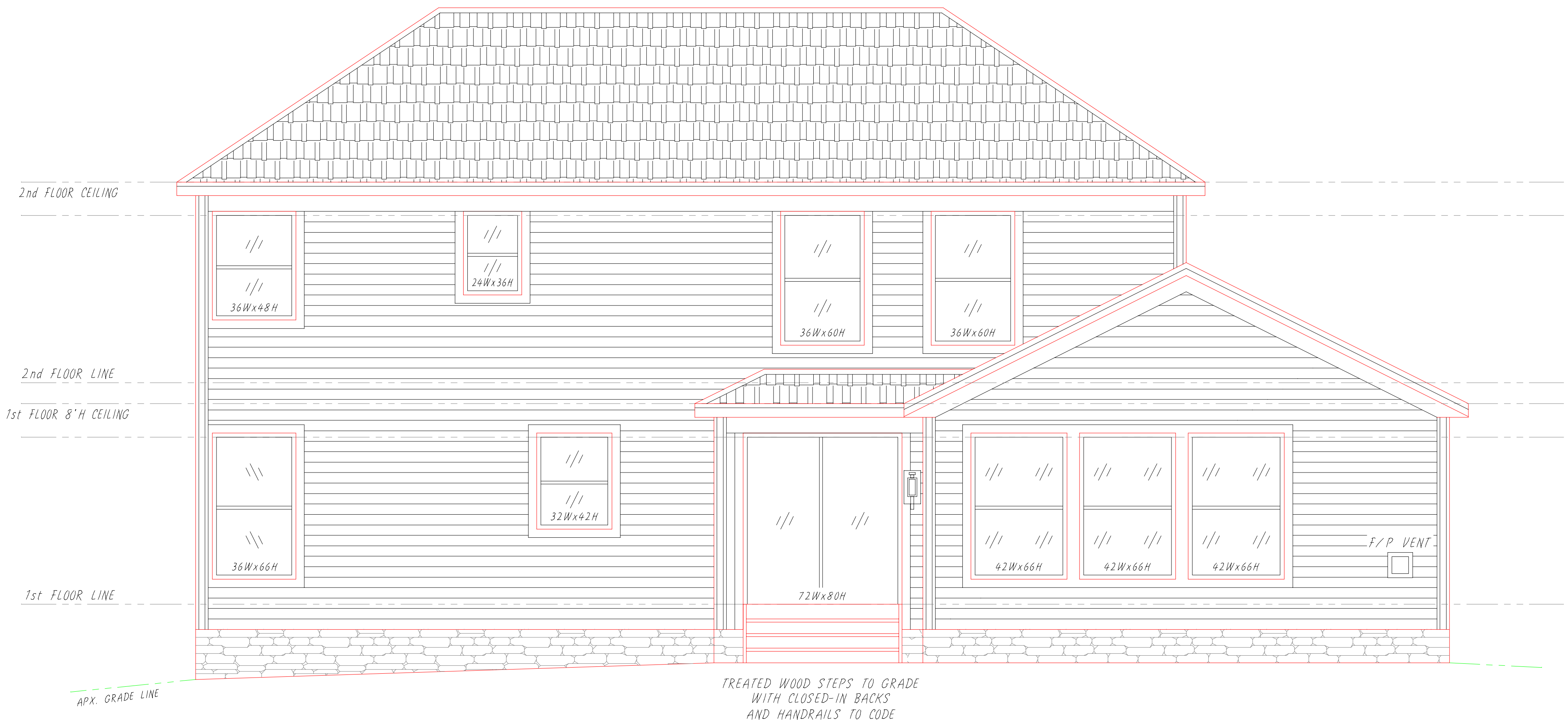
The Soulsby Residence Rear Elevation 090118
