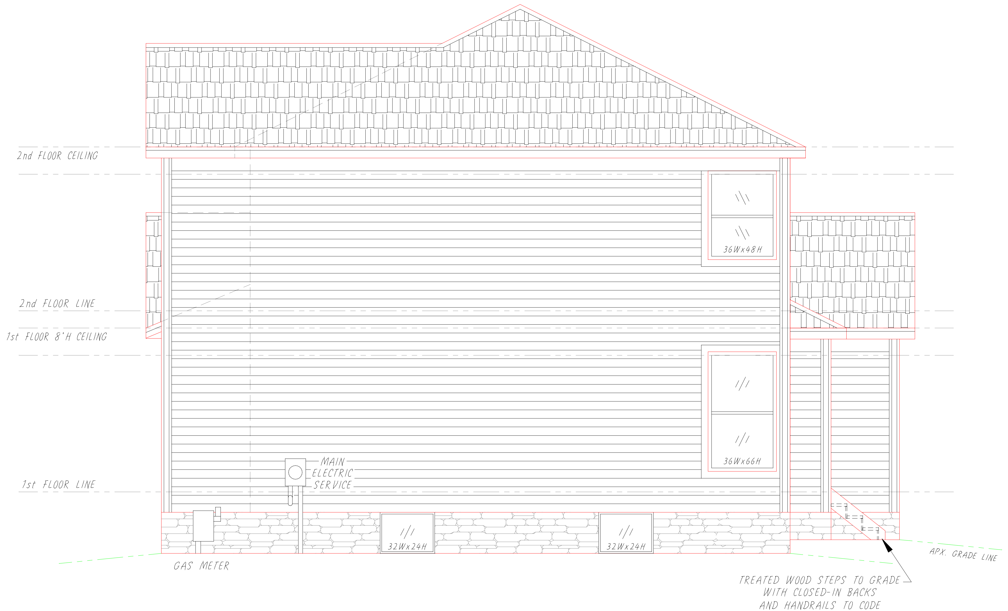
The Soulsby Residence Right Side Elevation 090118
