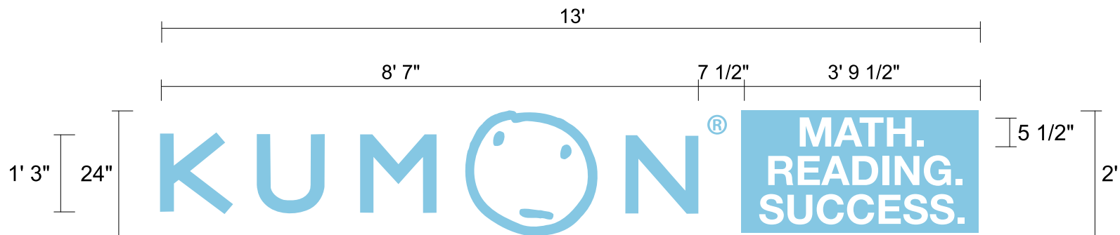
NORTH ELEVATION
