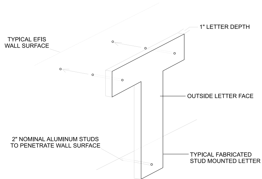
TYPICAL MOUNTING INSTALLATION TECHNIQUE FOR FABRICATED STUD MOUNTED LETTERS
