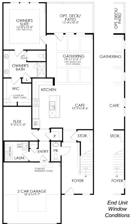
Addley Floorplan
