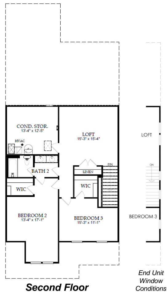
Addley Floorplan
