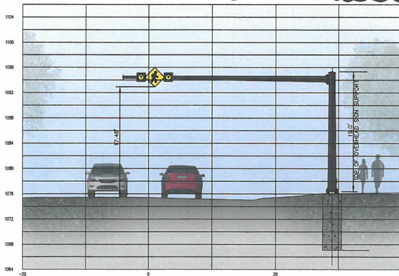
TRADITIONAL POLE WITH TRADITIONAL SIGNS ONLY
