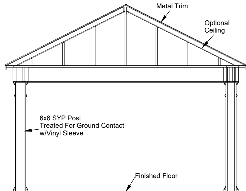
Cross Section Rafter
