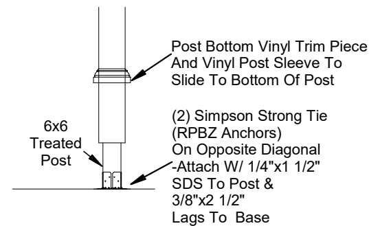
Post Anchor
