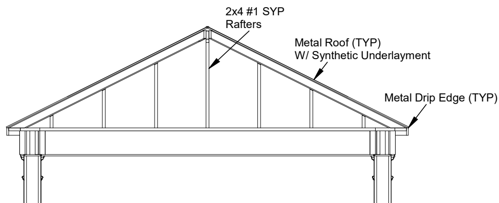
Rafter Detail
