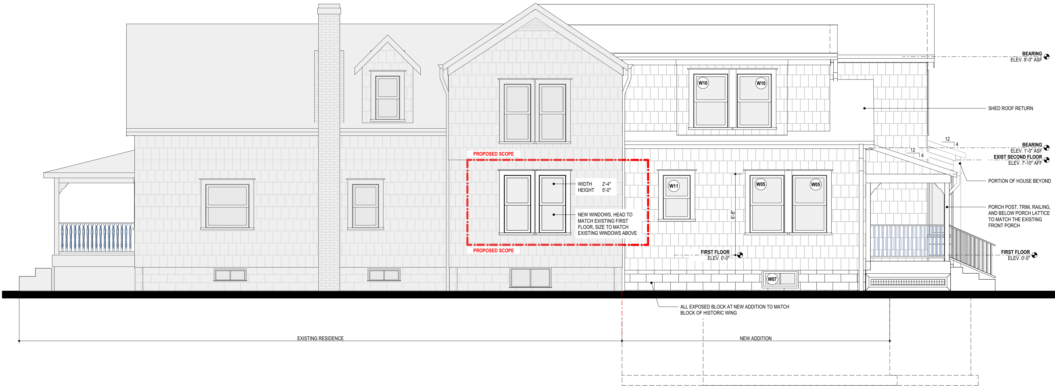
1 SOUTH ELEVATION (SIDE OF HOUSE) SCALE: 1/4" = 1'-0"
