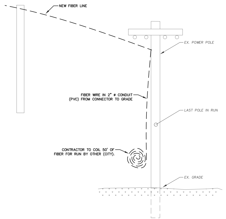
PROPOSED LAST POLE DETAIL NOT TO SCALE
