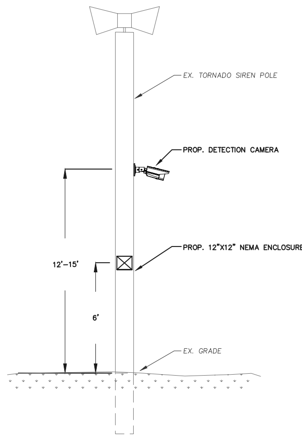
TORNADO SIREN POLE DETAIL NOT TO SCALE
