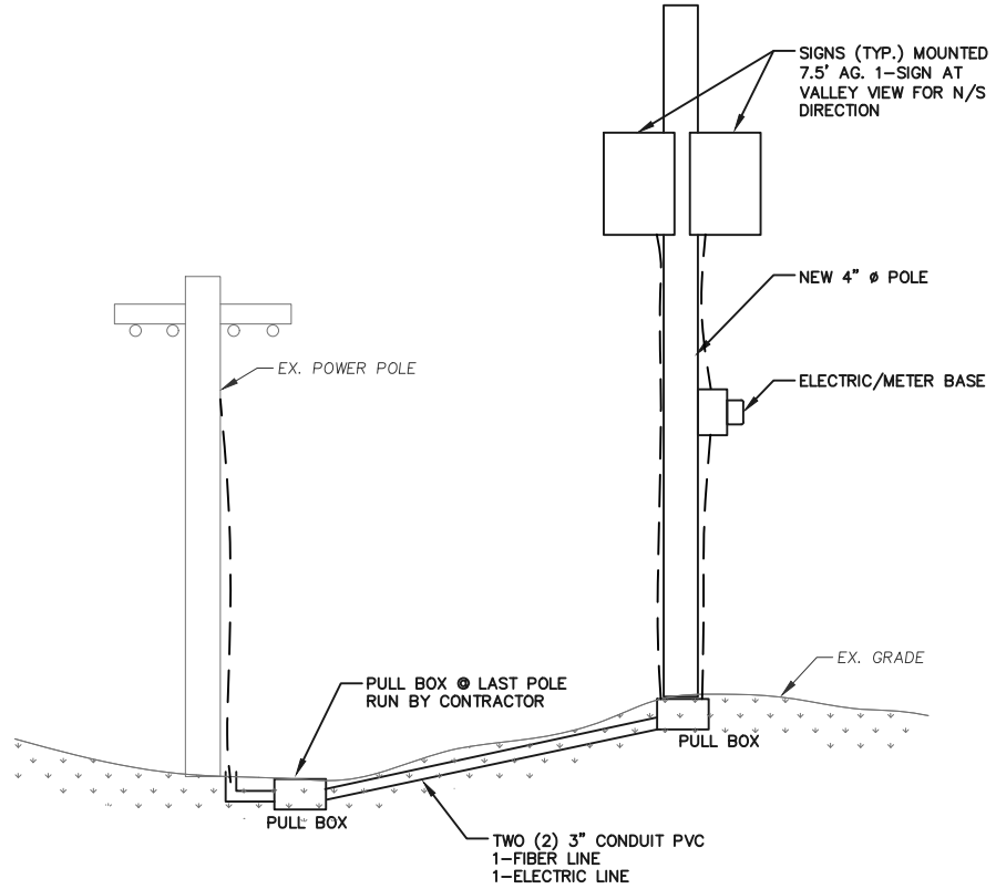
SIGN DETAIL NOT TO SCALE
