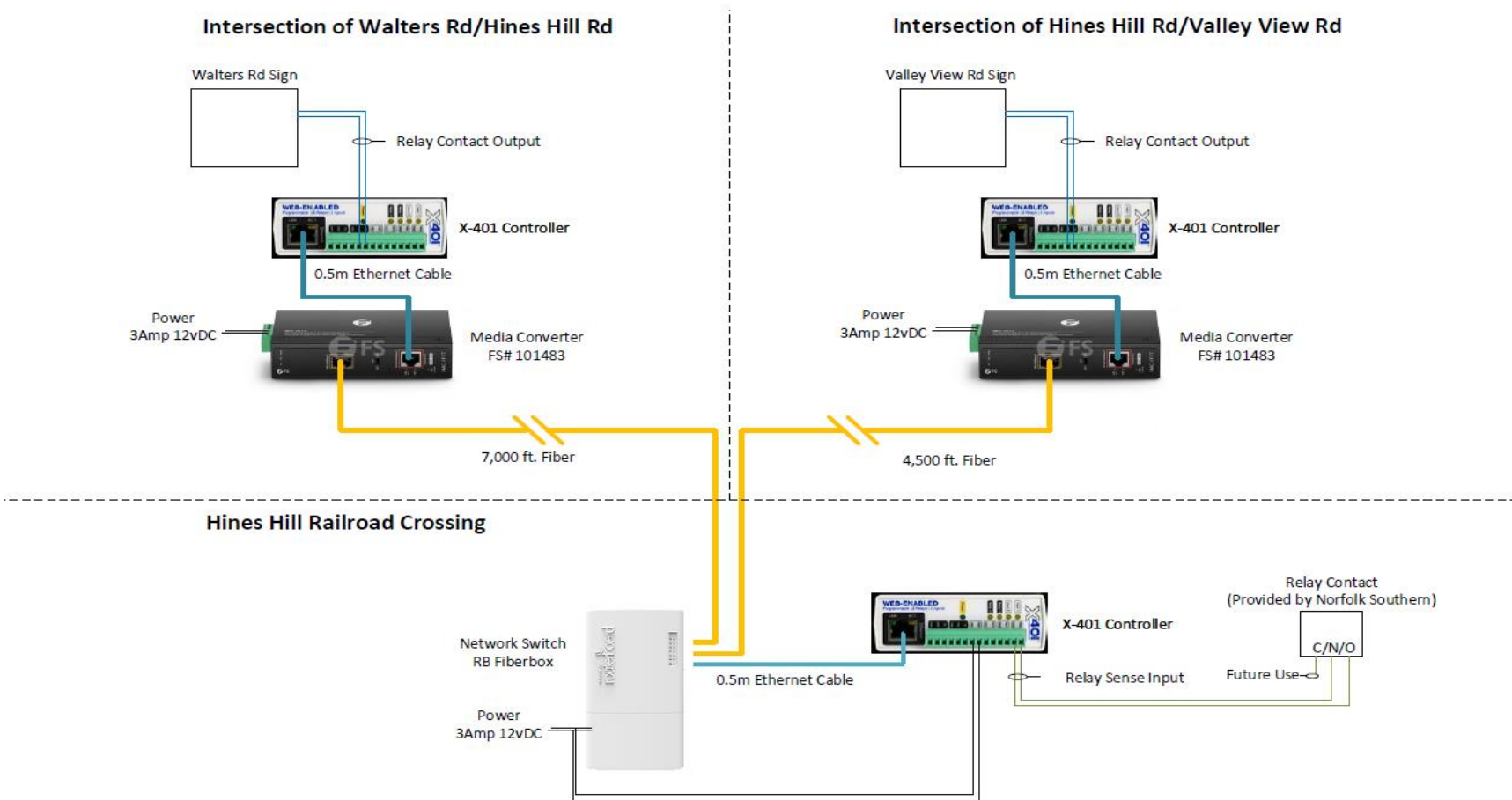
Proposed wiring diagram for Hines Hill RR Crossing
