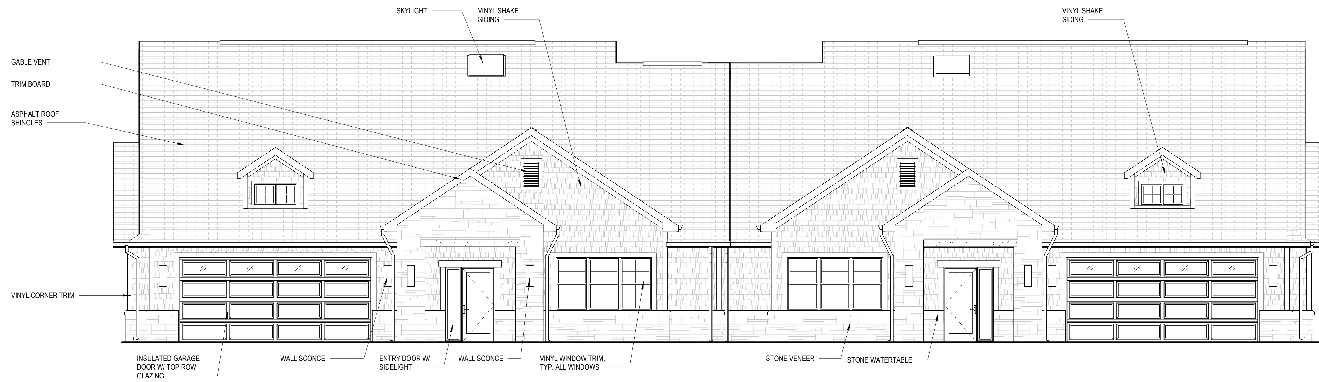
1 FRONT ELEVATION A201 3/16" = 1'-0"
