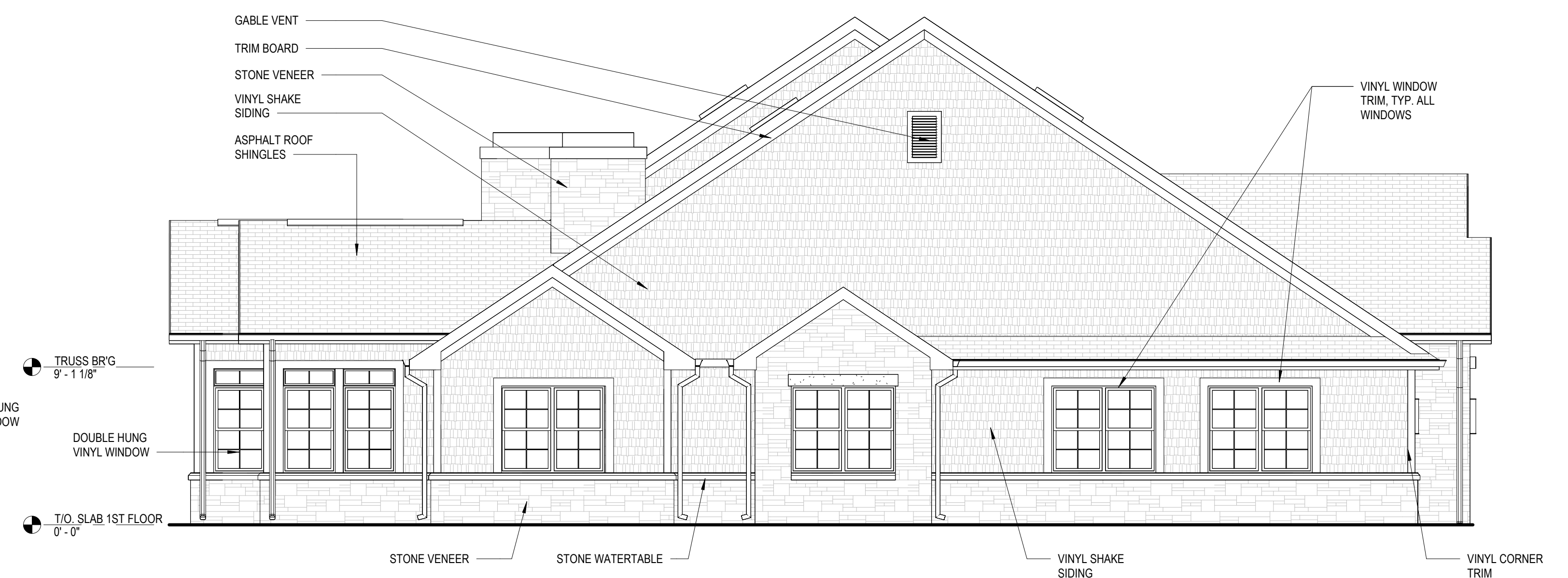
2 LEFT ELEVATION 3/16" = 1'-0"
