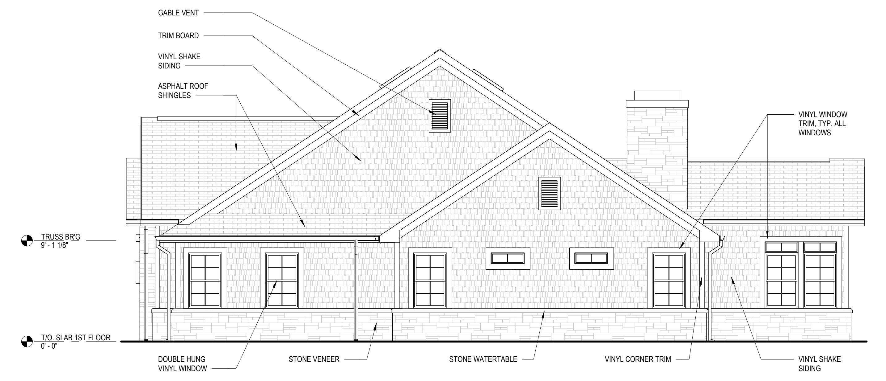
3 RIGHT ELEVATION A102 3/16" = 1'-0"
