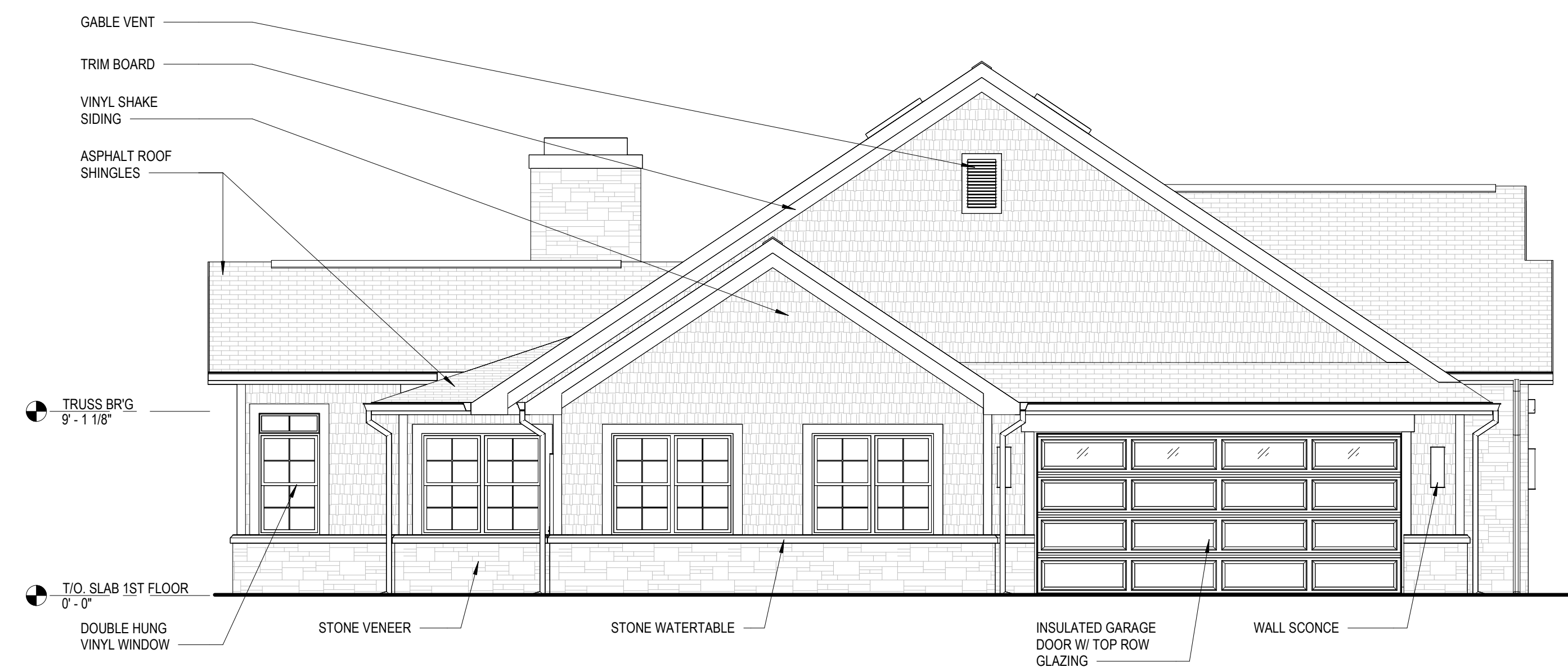
2 LEFT ELEVATION A102 3/16" = 1'-0"
