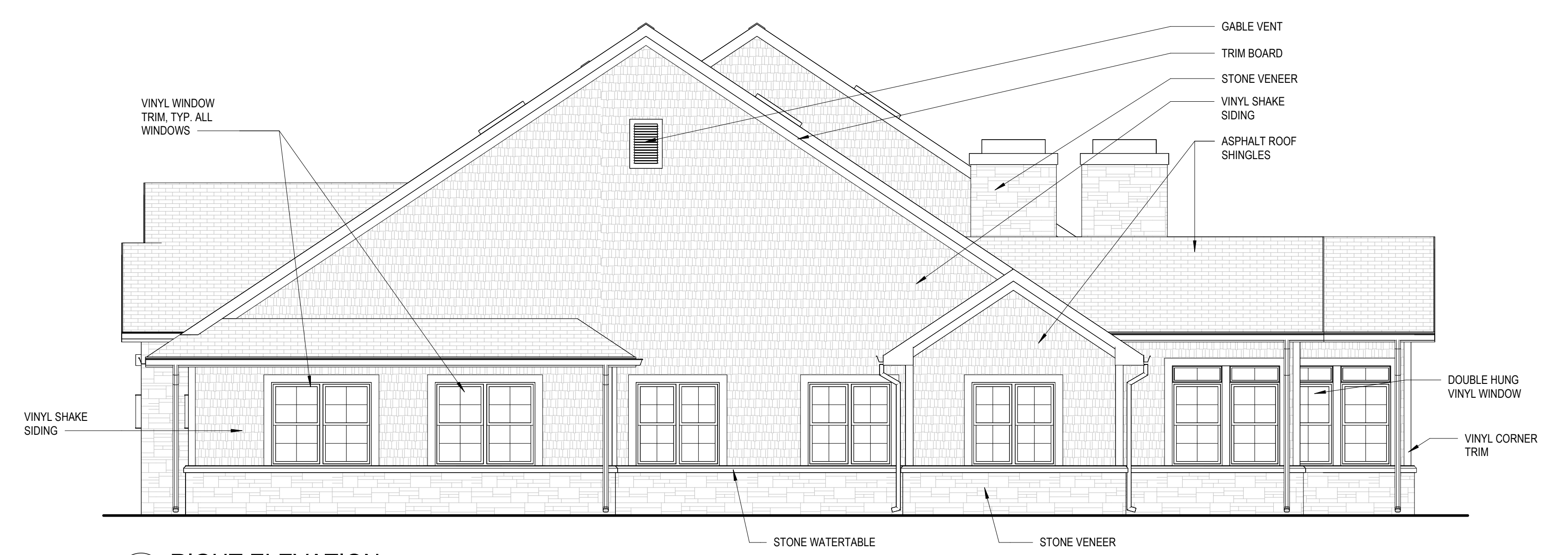
2 RIGHT ELEVATION A201 3/16" = 1'-0"
