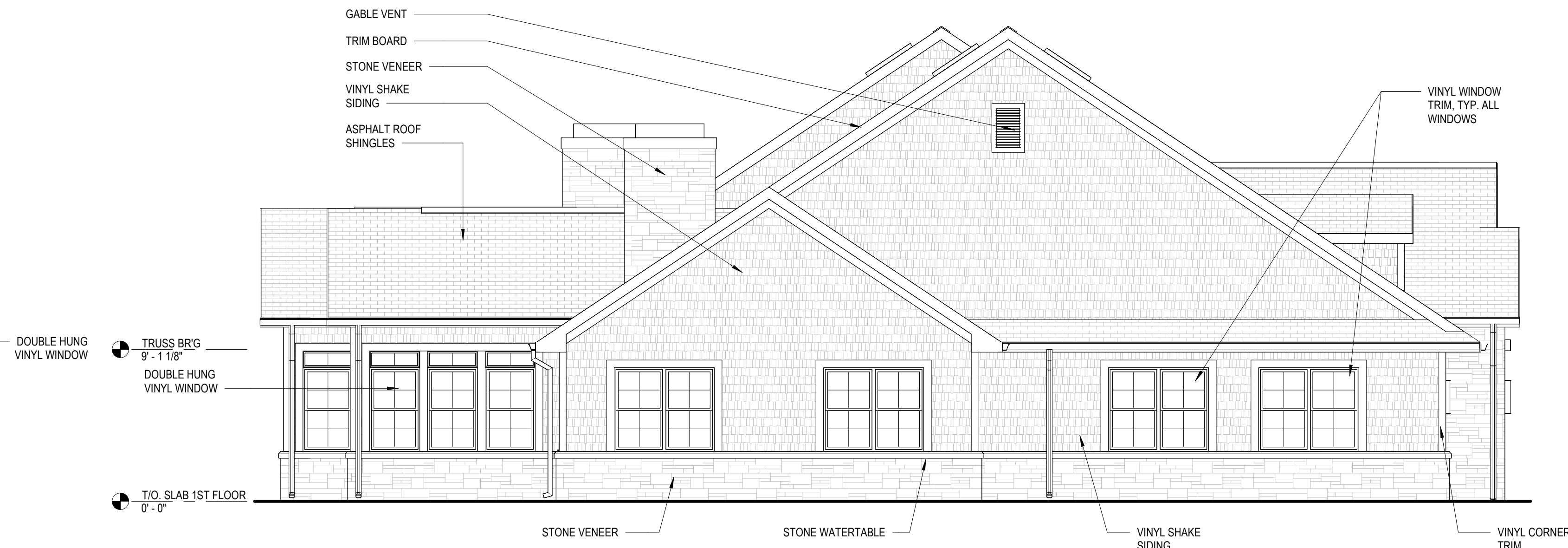
2 LEFT ELEVATION A201 3/16" = 1'-0"
