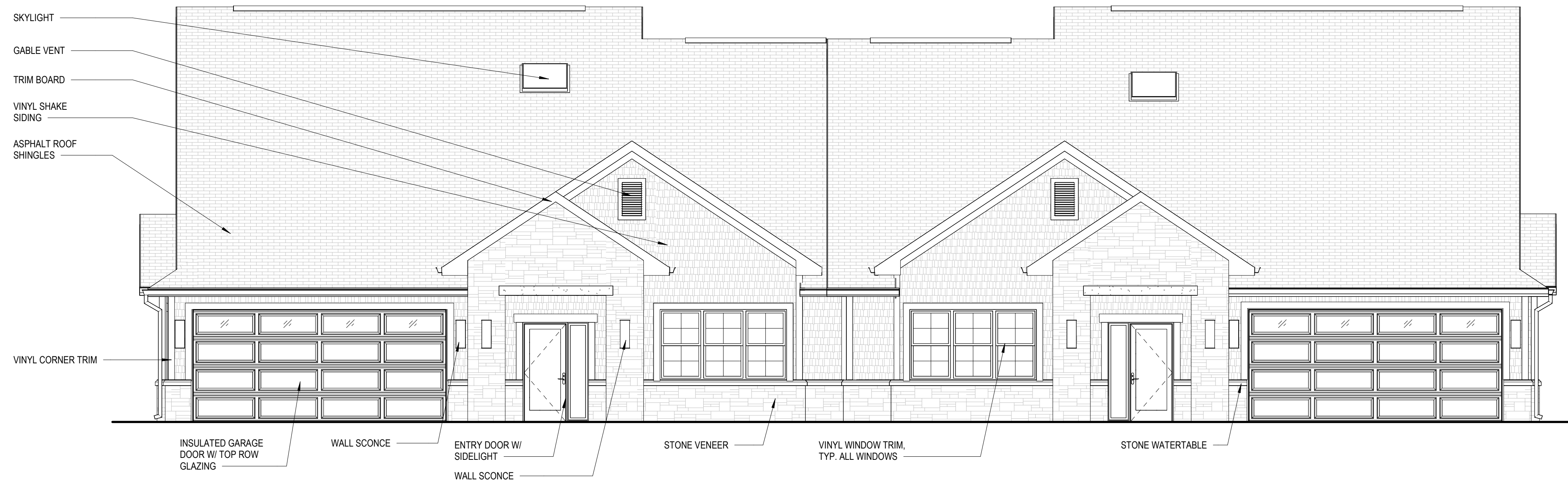
1 FRONT ELEVATION A201 3/16" = 1'-0"
