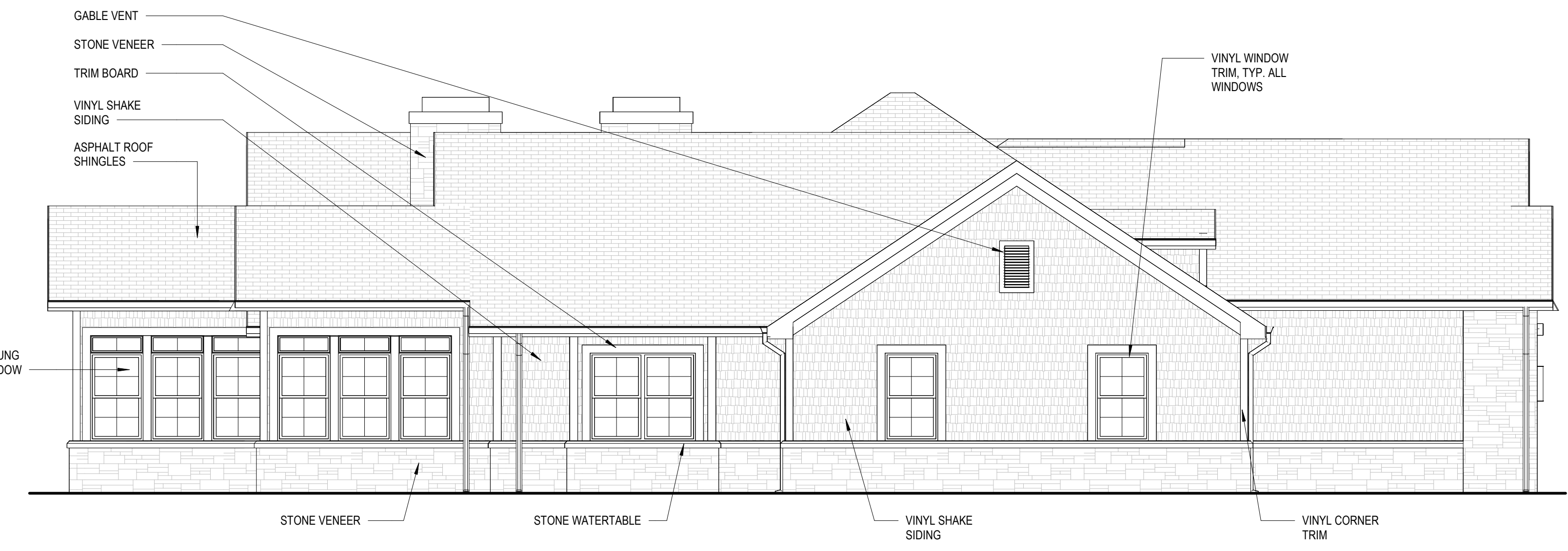
2 LEFT ELEVATION A201 3/16" = 1'-0"
