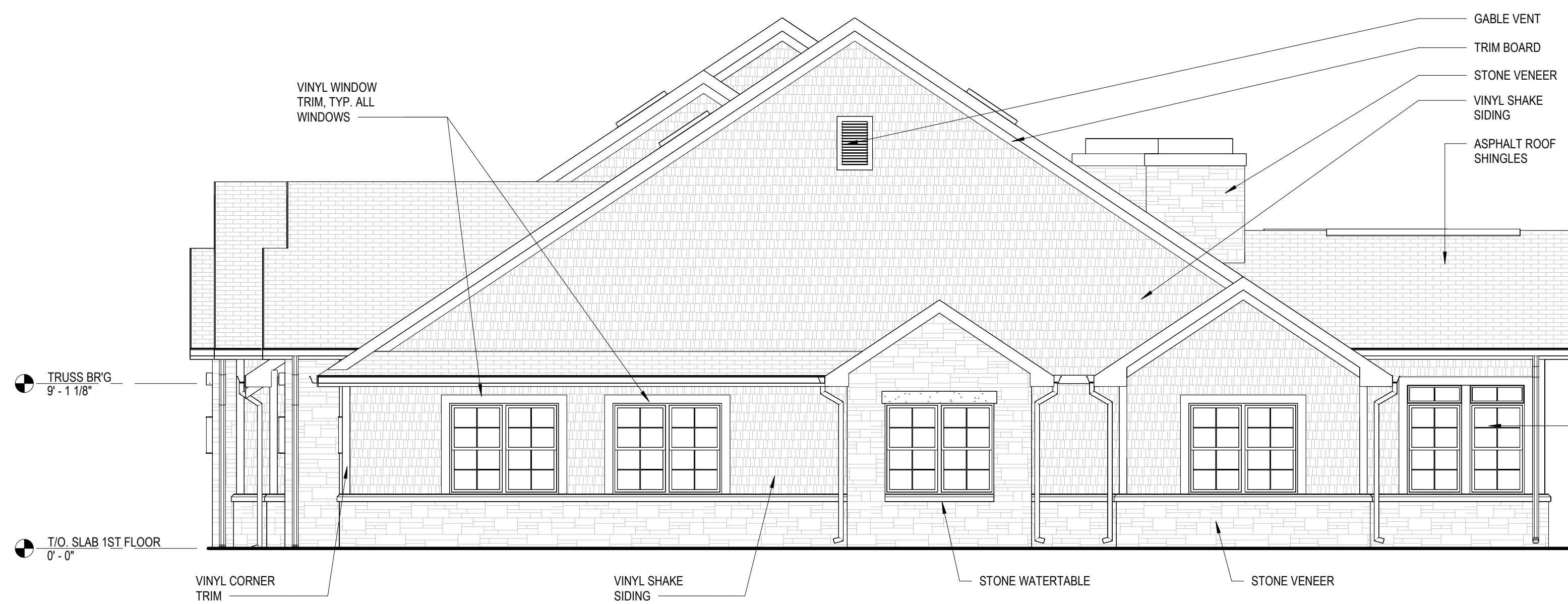
3 RIGHT ELEVATION 3/16" = 1'-0"
