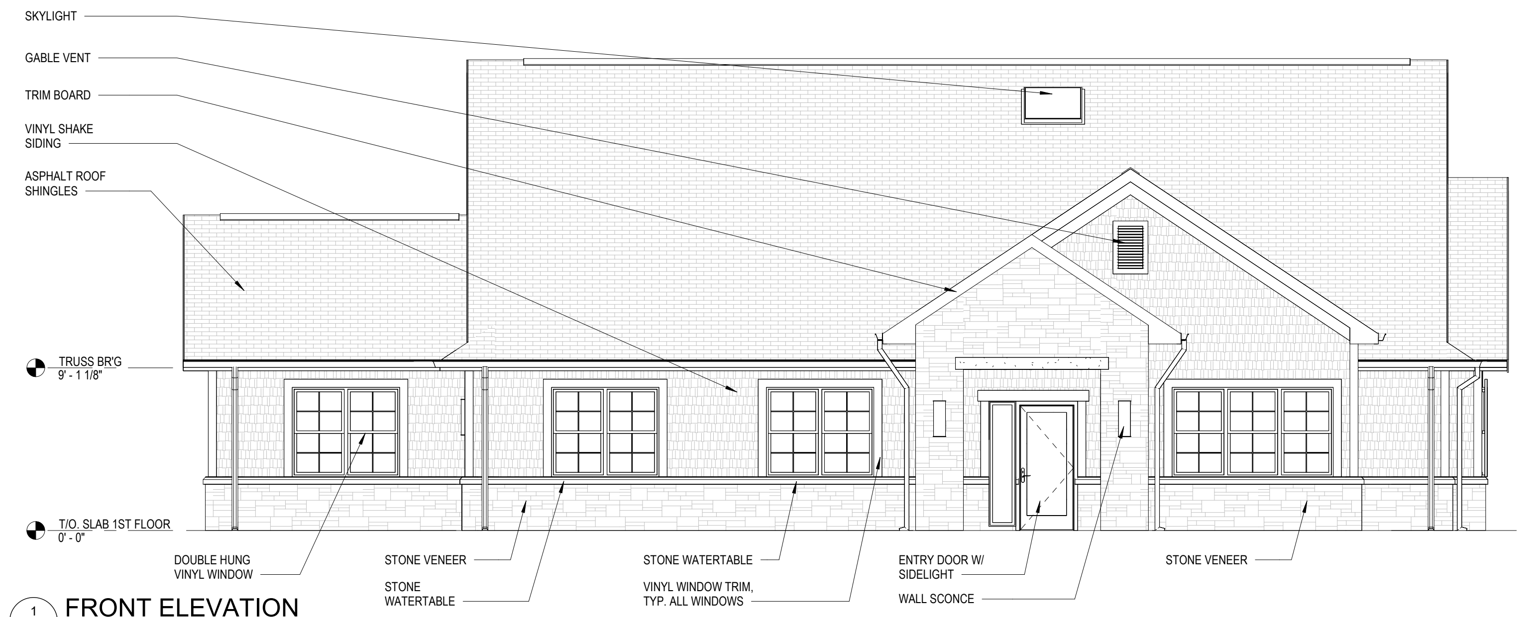
1 FRONT ELEVATION A102 3/16" = 1'-0"
