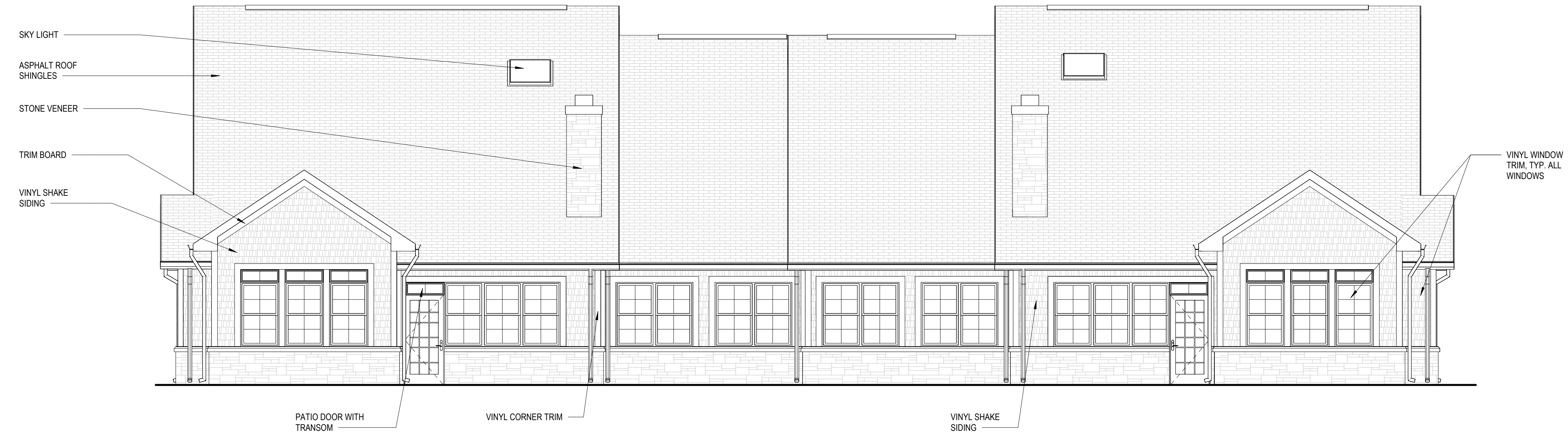
4 REAR ELEVATION A201 3/16" = 1'-0"
