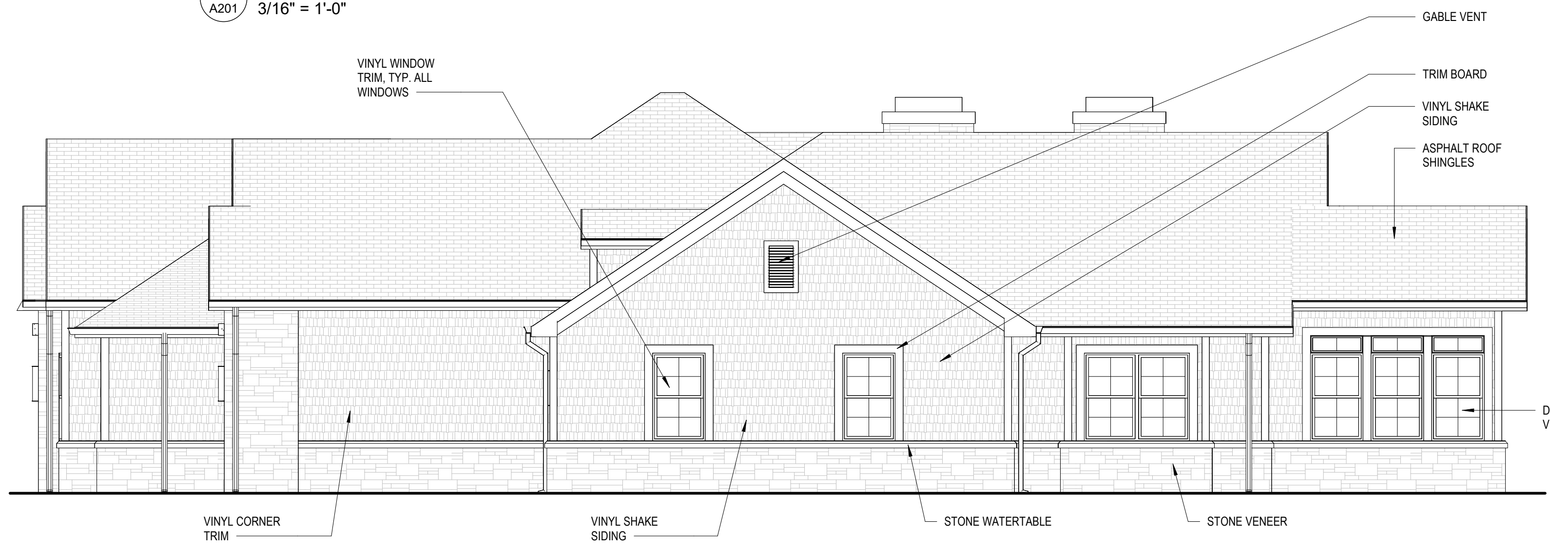
3 RIGHT ELEVATION A201 3/16" = 1'-0"
