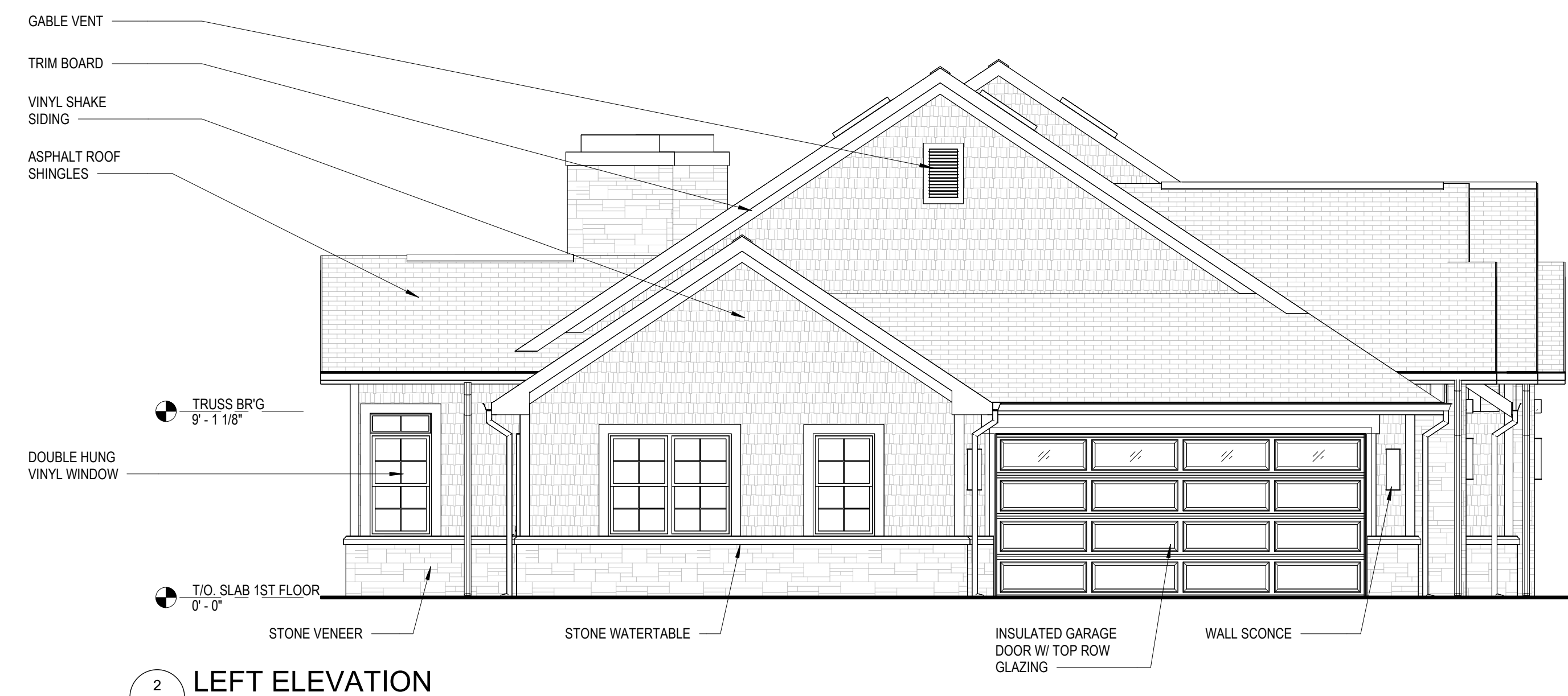
2 LEFT ELEVATION 3/16" = 1'-0"
