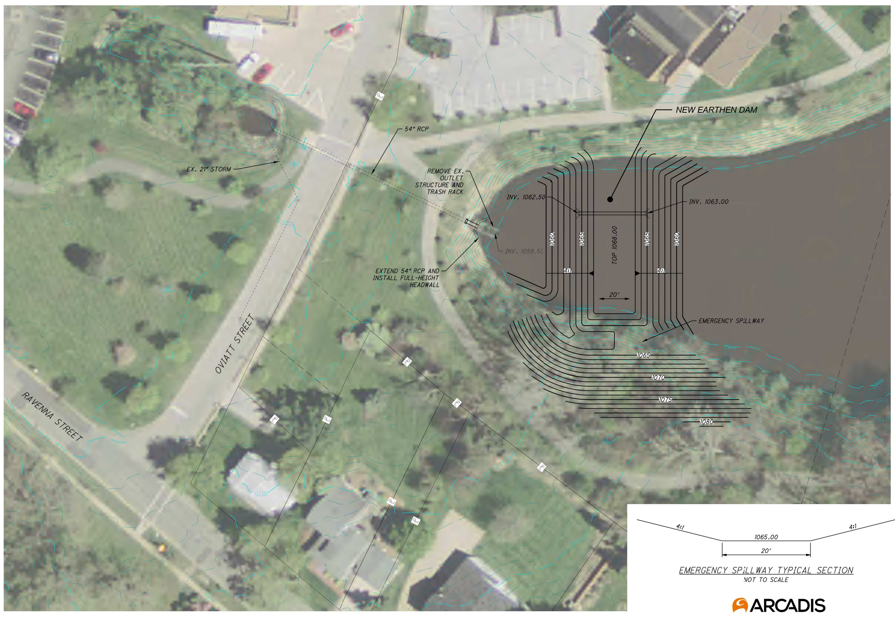
FIGURE 4 - WEST POND (LOWER LAKE) DAM ALTERNATIVE B
