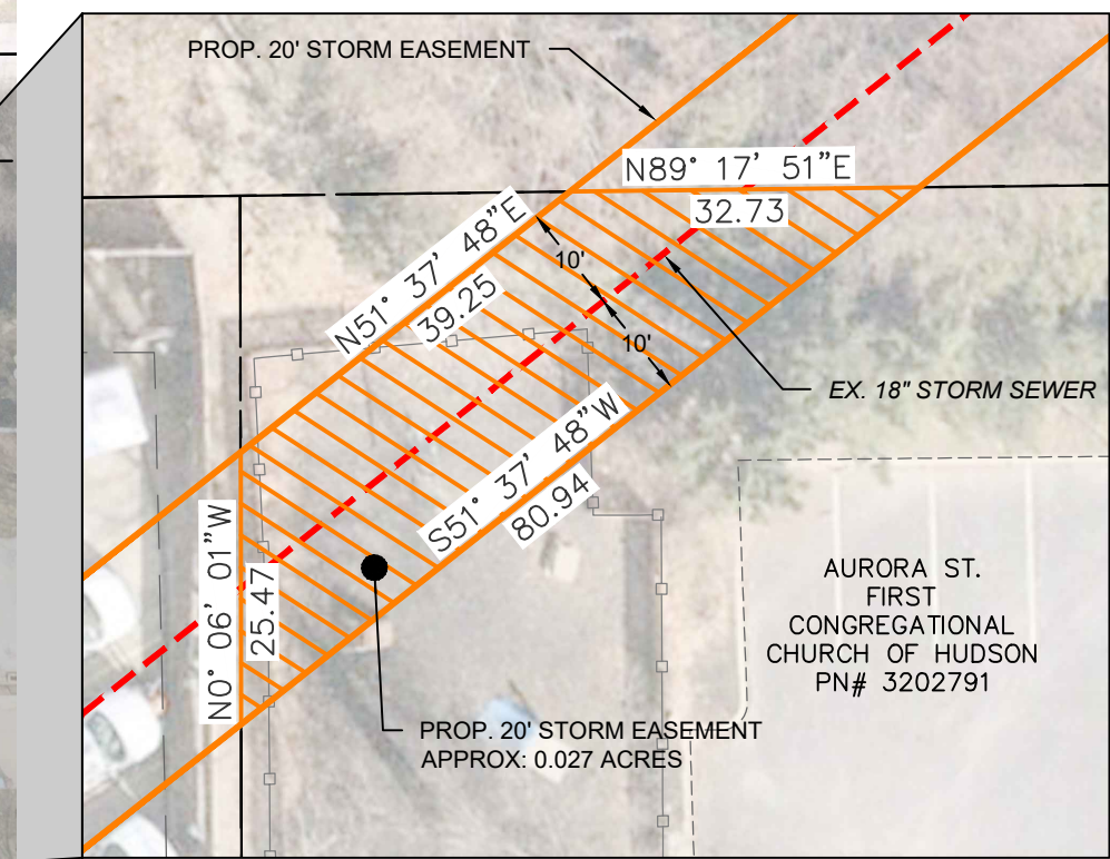
FIRST CONGREGATIONAL CHURCH OF HUDSON EASEMENT DETAIL
