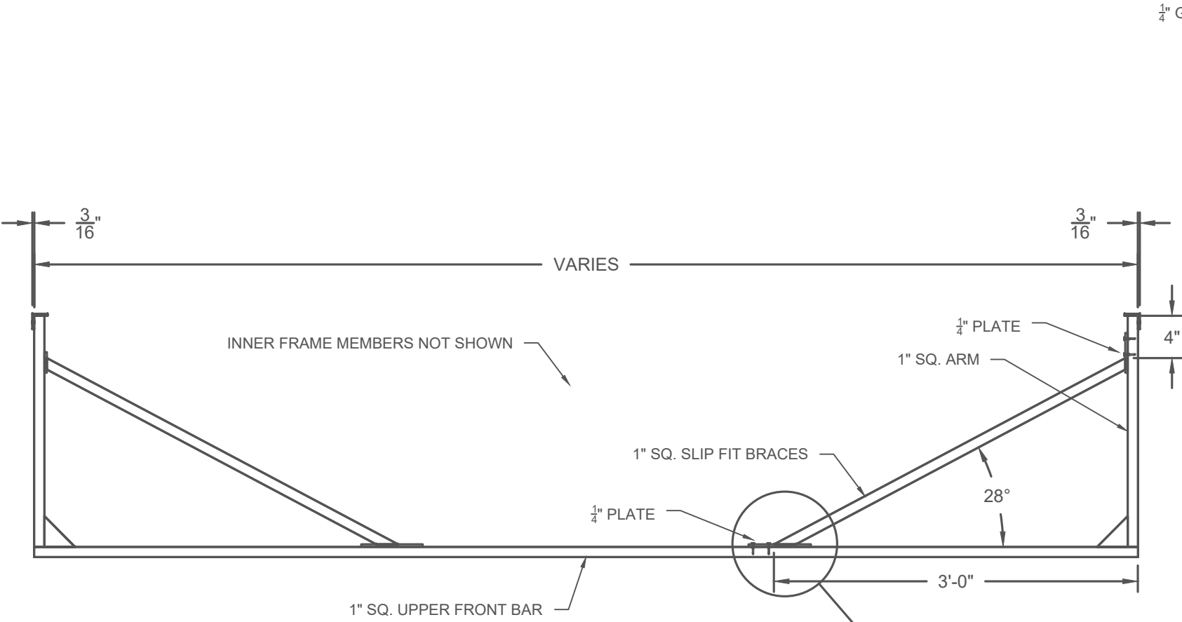
AWNING FRAME TOP VIEW SLIP FIT BRACES FRAMES #1 & #6
