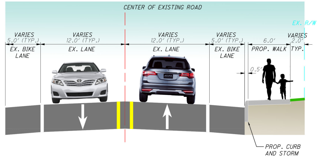
SR 303 - NORTH HAYDEN PARKWAY TO STONE ROAD STOW ROAD - SR 303 TO HUDSON SPRINGS PARK (SHOWN PER DIRECTION OF TRAVEL, REVERSE AS NECESSARY) CURB SECTION - NO TREE LAWN
