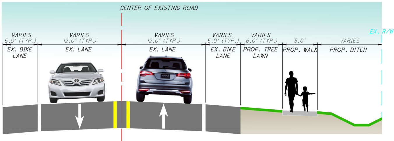
SR 303 - NORTH HAYDEN PARKWAY TO STONE ROAD STOW ROAD - SR 303 TO HUDSON SPRINGS PARK (SHOWN PER DIRECTION OF TRAVEL, REVERSE AS NECESSARY) DITCH SECTION
