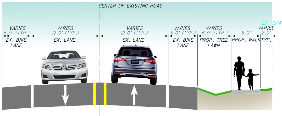
PREFERRED TYPICAL SECTION SR 303 - NORTH HAYDEN PARKWAY TO STONE ROAD STOW ROAD - SR 303 TO HUDSON SPRINGS PARK (SHOWN PER DIRECTION OF TRAVEL, REVERSE AS NECESSARY) SWALE SECTION
