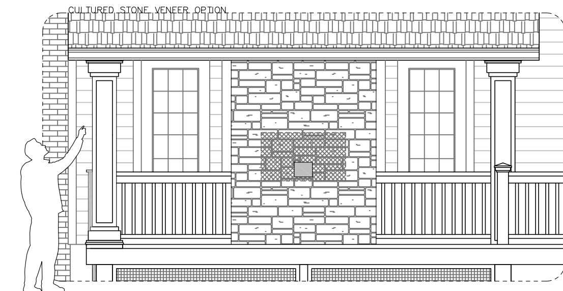
2a ALTERNATE ELEVATION w/ stone veneer SCALE 1/4" = 1'-0"
