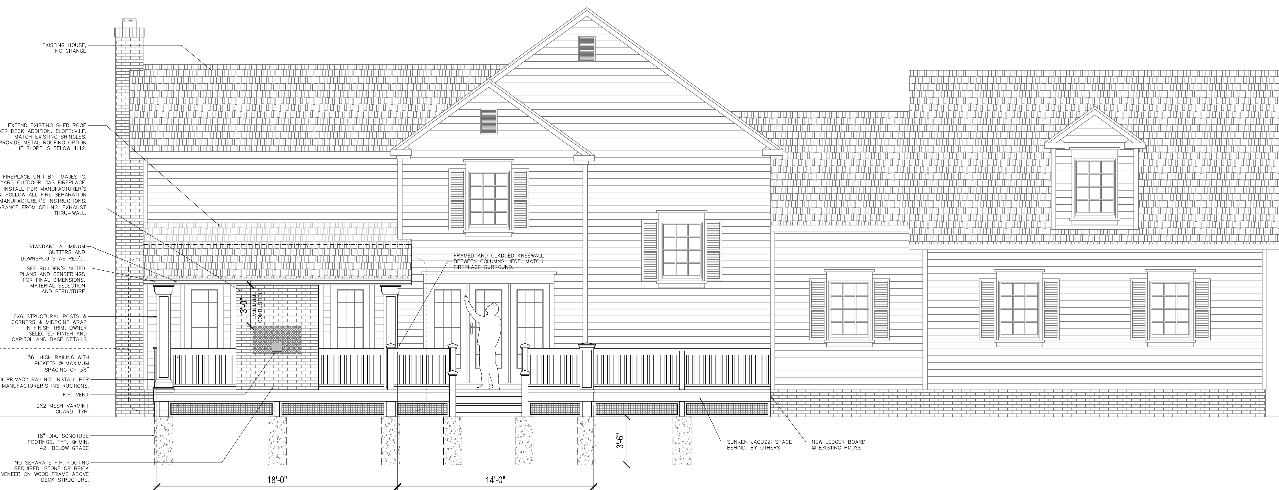
2 PROPOSED REAR ELEVATION SCALE 1/4" = 1'-0"
