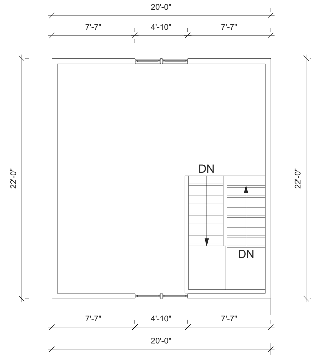
Second Floor
