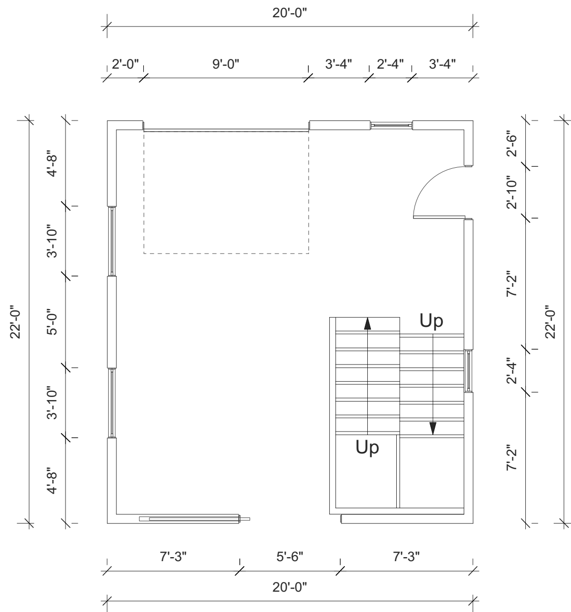
First Floor
