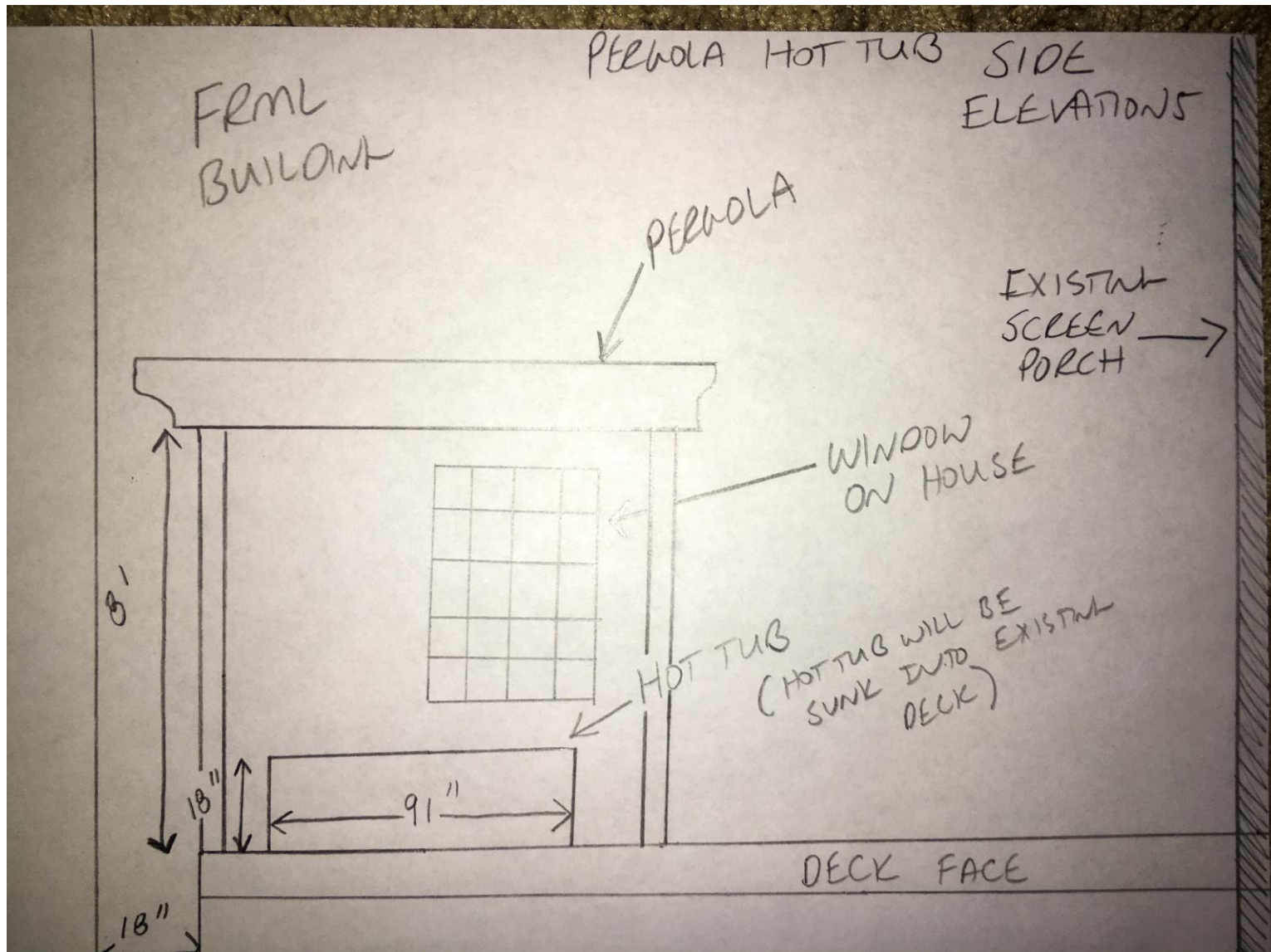
DIBIASIO Pergola Hot Tub Side Elevation
