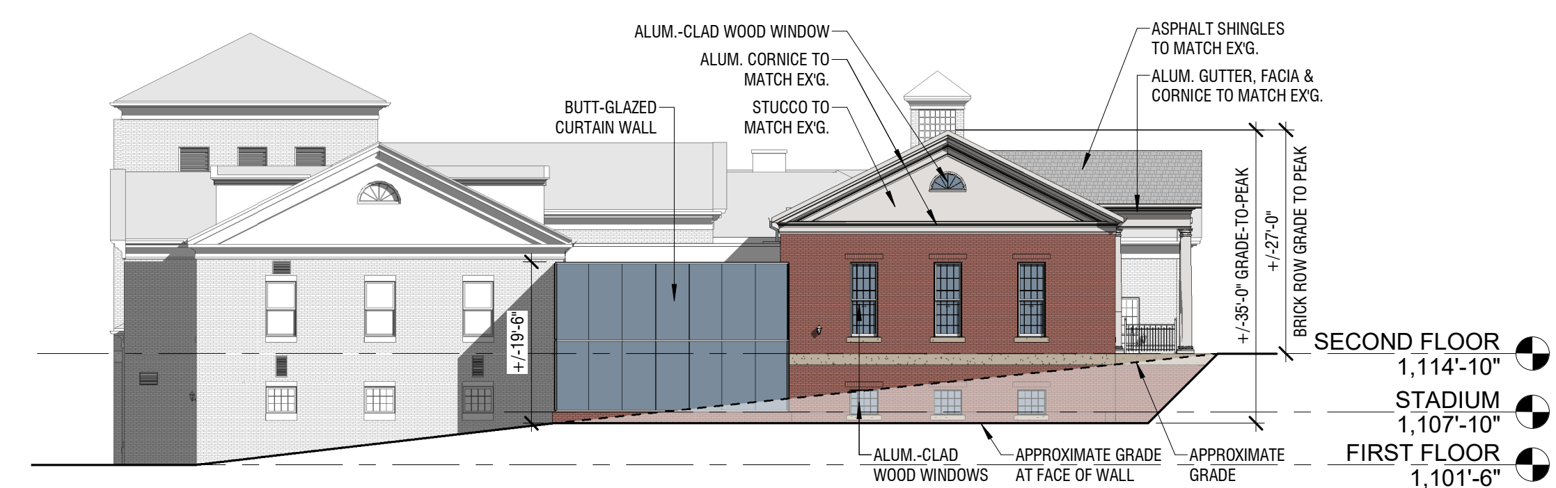
② PROPOSED NORTH ELEVATION 1/16" = 1'-0"
