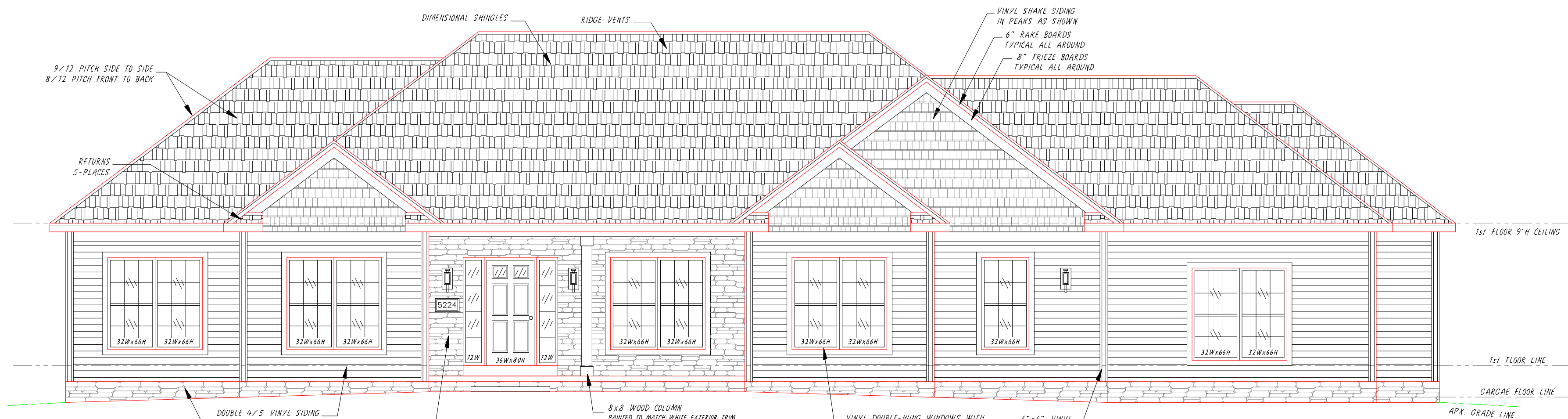
Front Elevation (S/L 3 - 5224 Preserve Lane)
