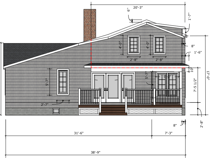
NORTH ELEVATION (REAR OF HOUSE)
