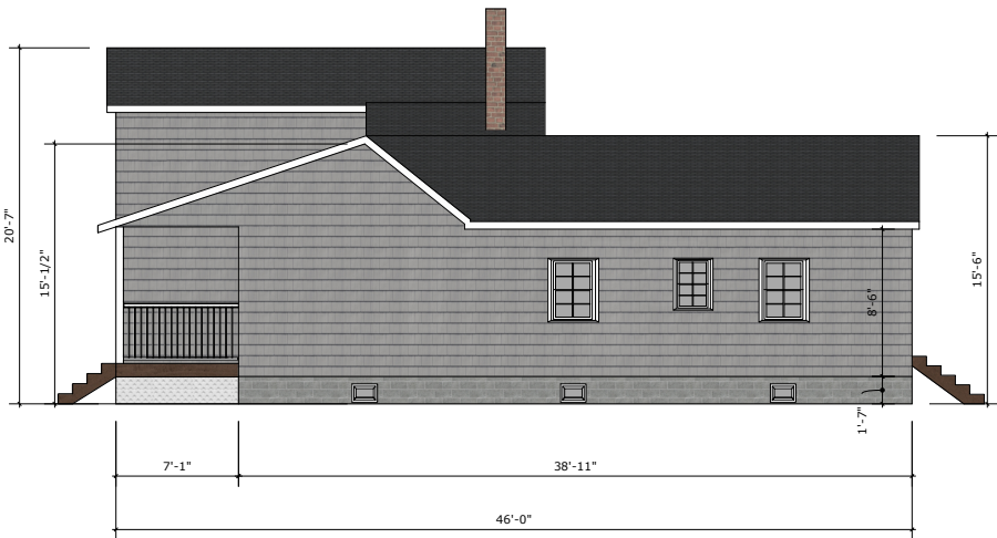
EAST (SIDE OF HOUSE)
