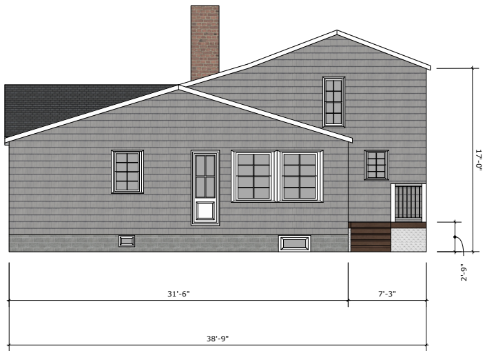
NORTH ELEVATION (REAR OF HOUSE)
