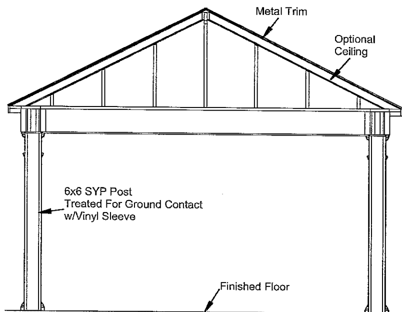
Cross Section Rafters
