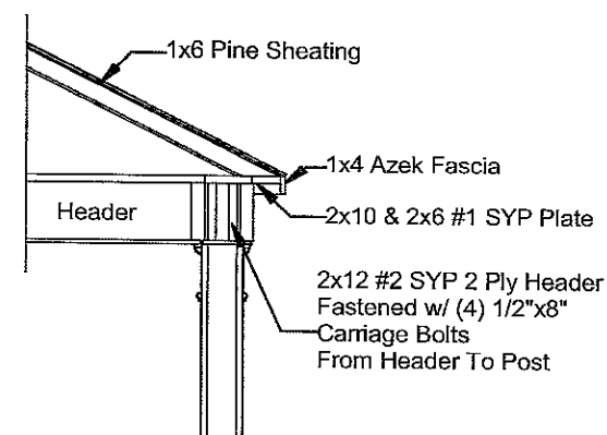
2x10 Header Connection Detail
