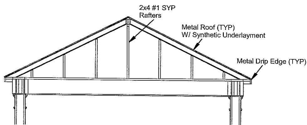
Rafter Detail
