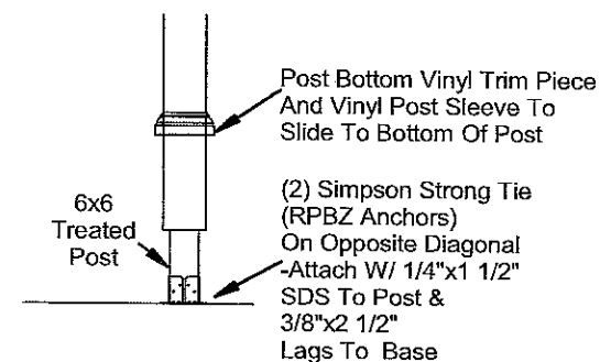
Post Anchor
