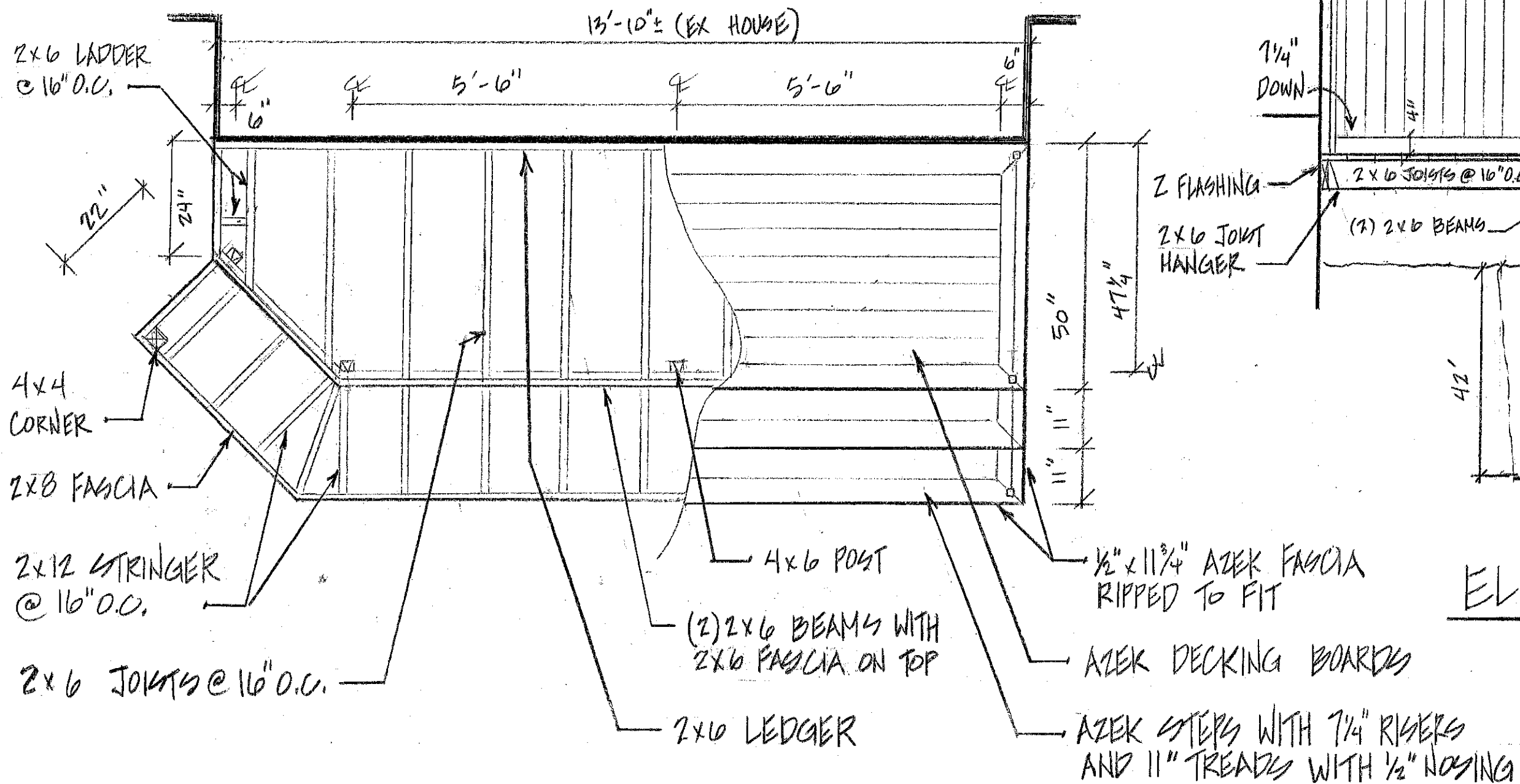
PLAN VIEW
