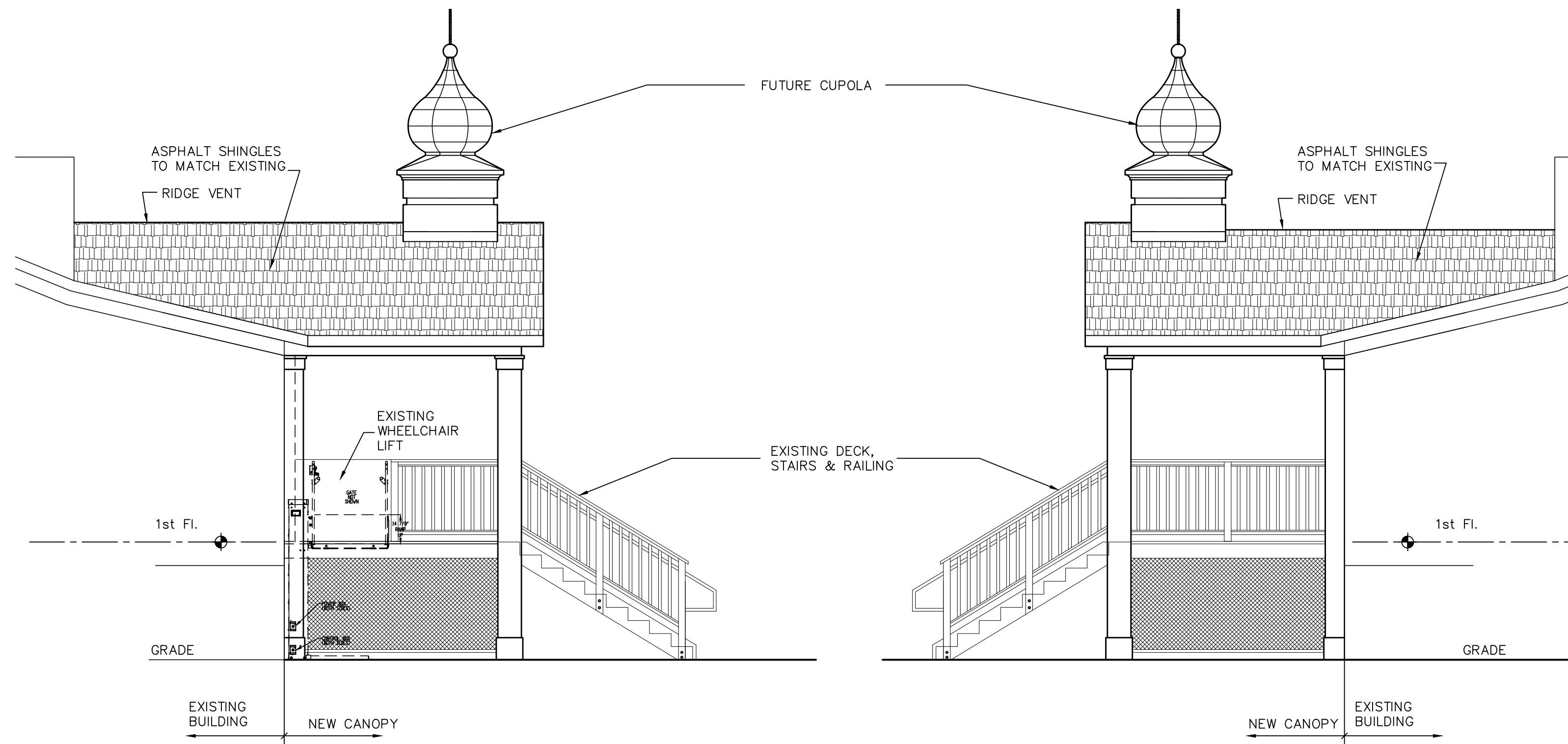
3 SOUTH ELEVATION SK1.2 1/4" = 1'-0"
