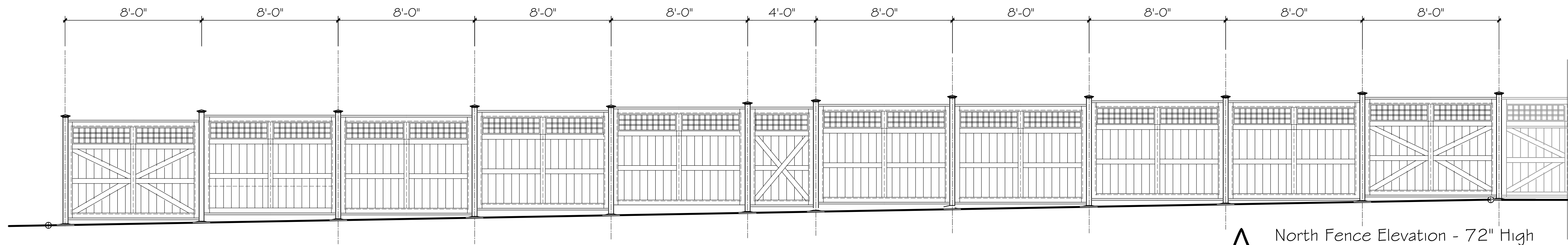
A North Fence Elevation - 72" High Scale: 1/4"=1'-0"
