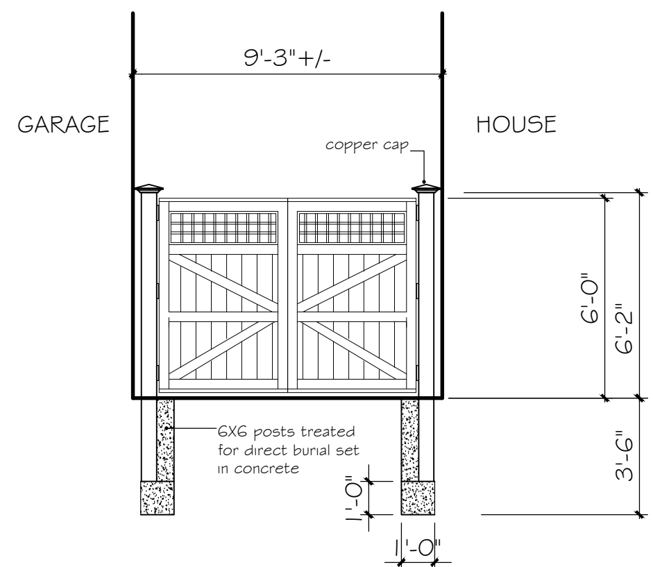
F Garden Gate - 72" High Scale: 1/4"=1'-0"
