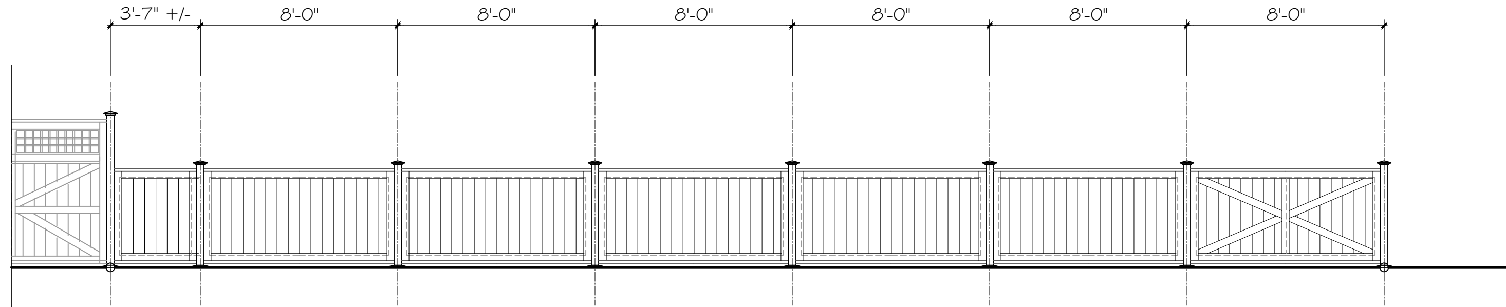
B North Fence Elevation - 48" High Scale: 1/4"=1'-0"
