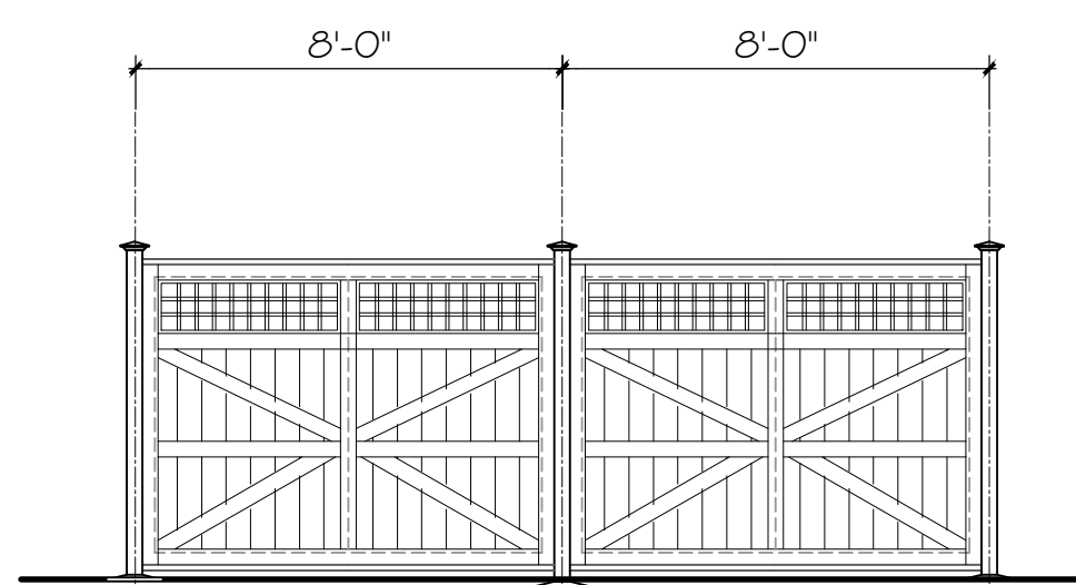
C North Fence Elevation - 72" High Scale: 1/4"=1'-0"
