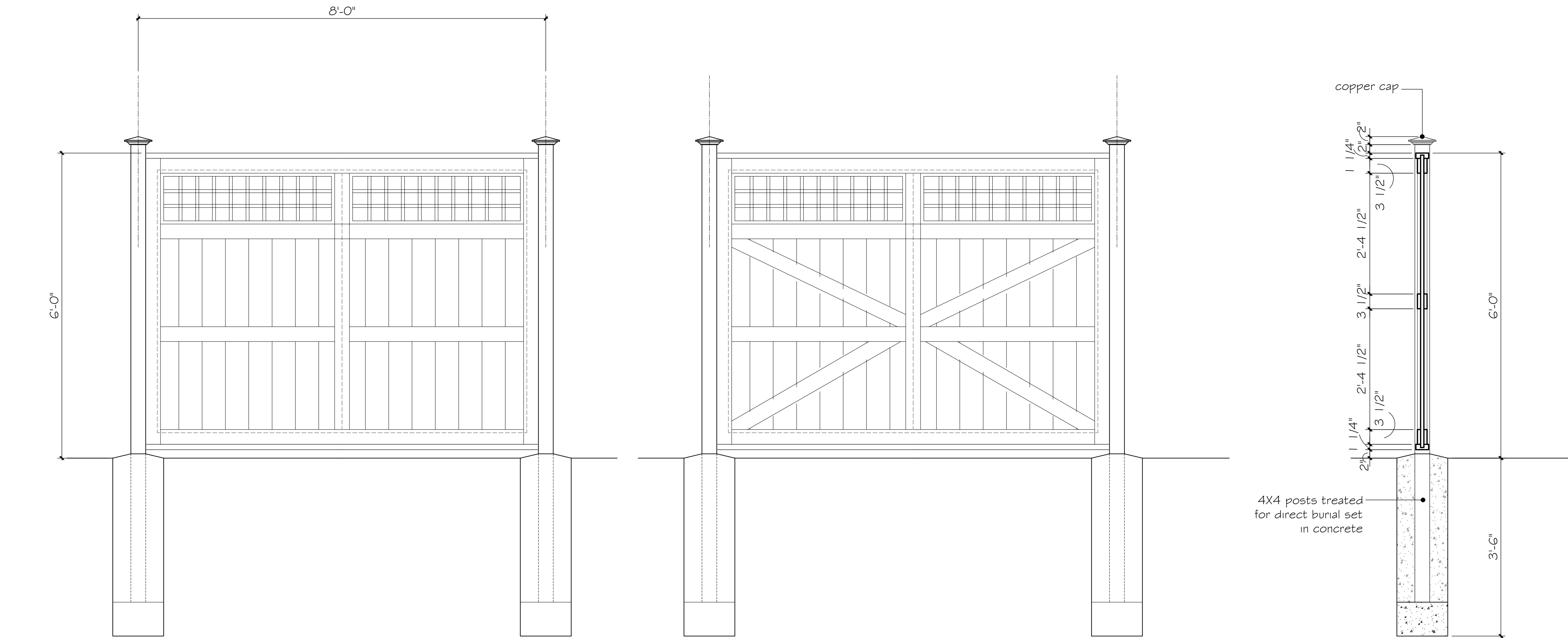
Fence Elevation - 72" High Scale: 3/4"= 1'-0"
