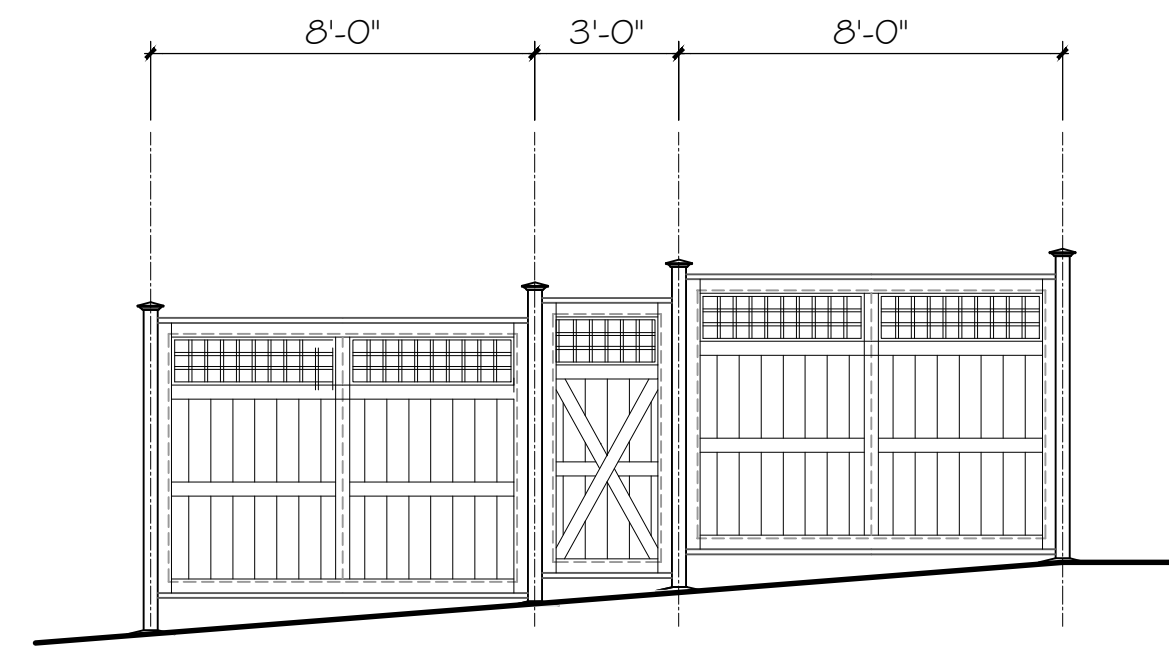
D North Fence Elevation - 72" High Scale: 1/4"=1'-0"
