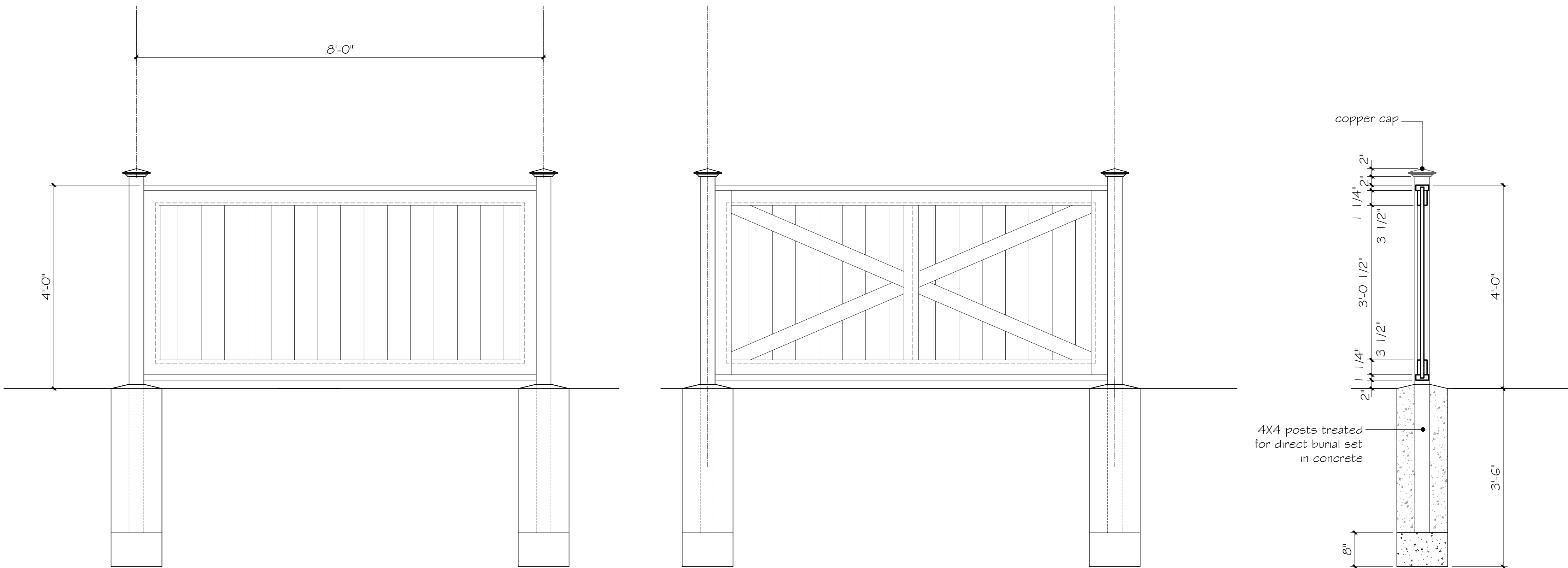
Fence Elevation - 48" High Scale: 3/4"= 1'-0"
