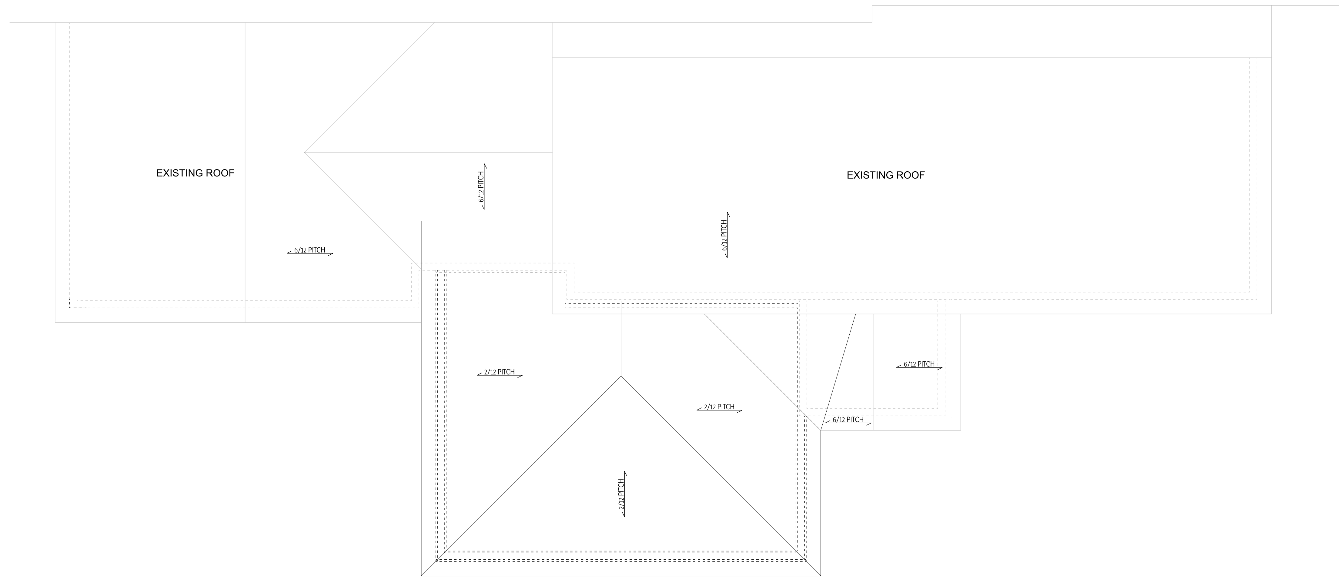
ROOF PLAN SCALE: 1/4" = 1'-0"
