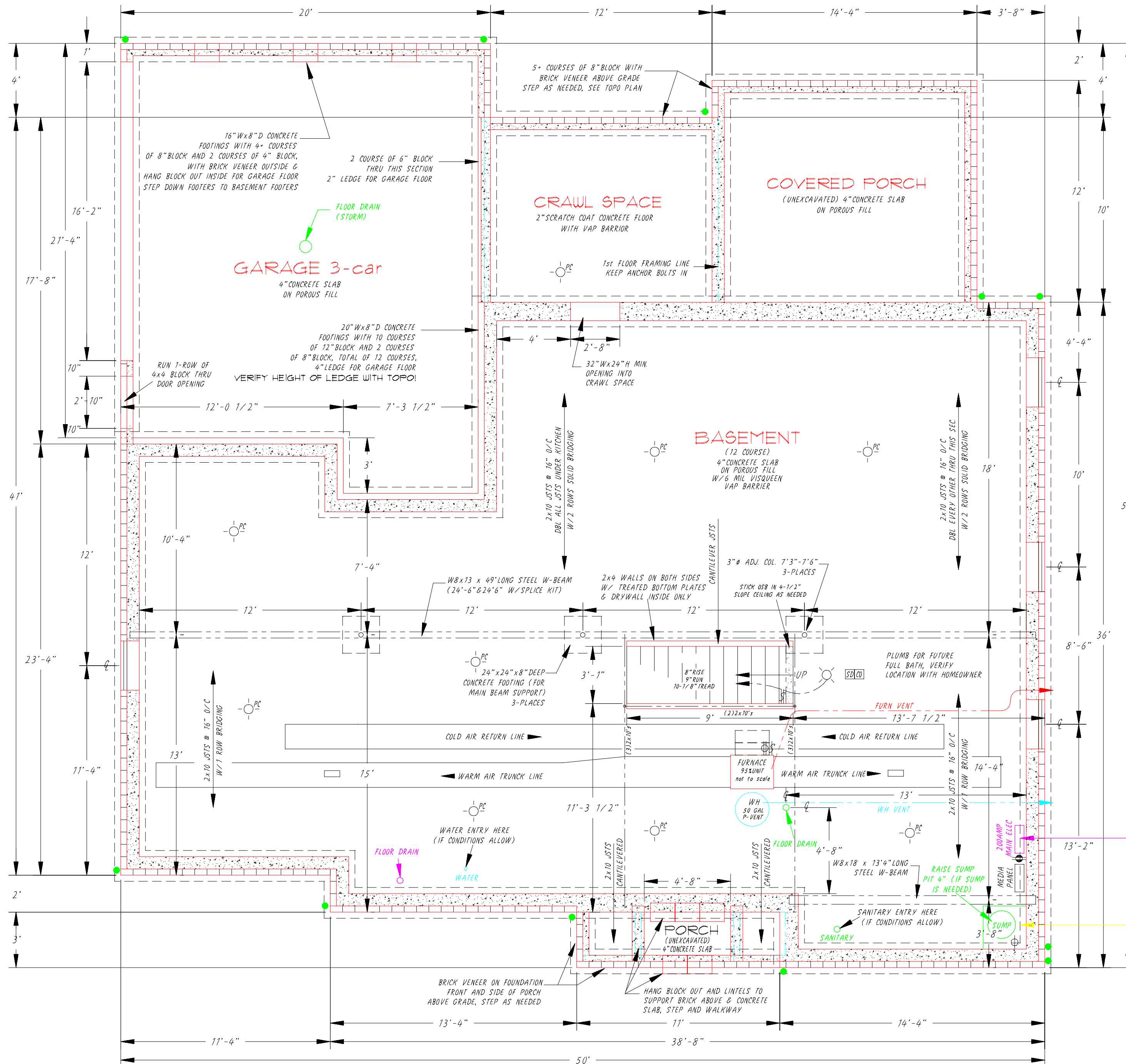
Foundation Front of House
