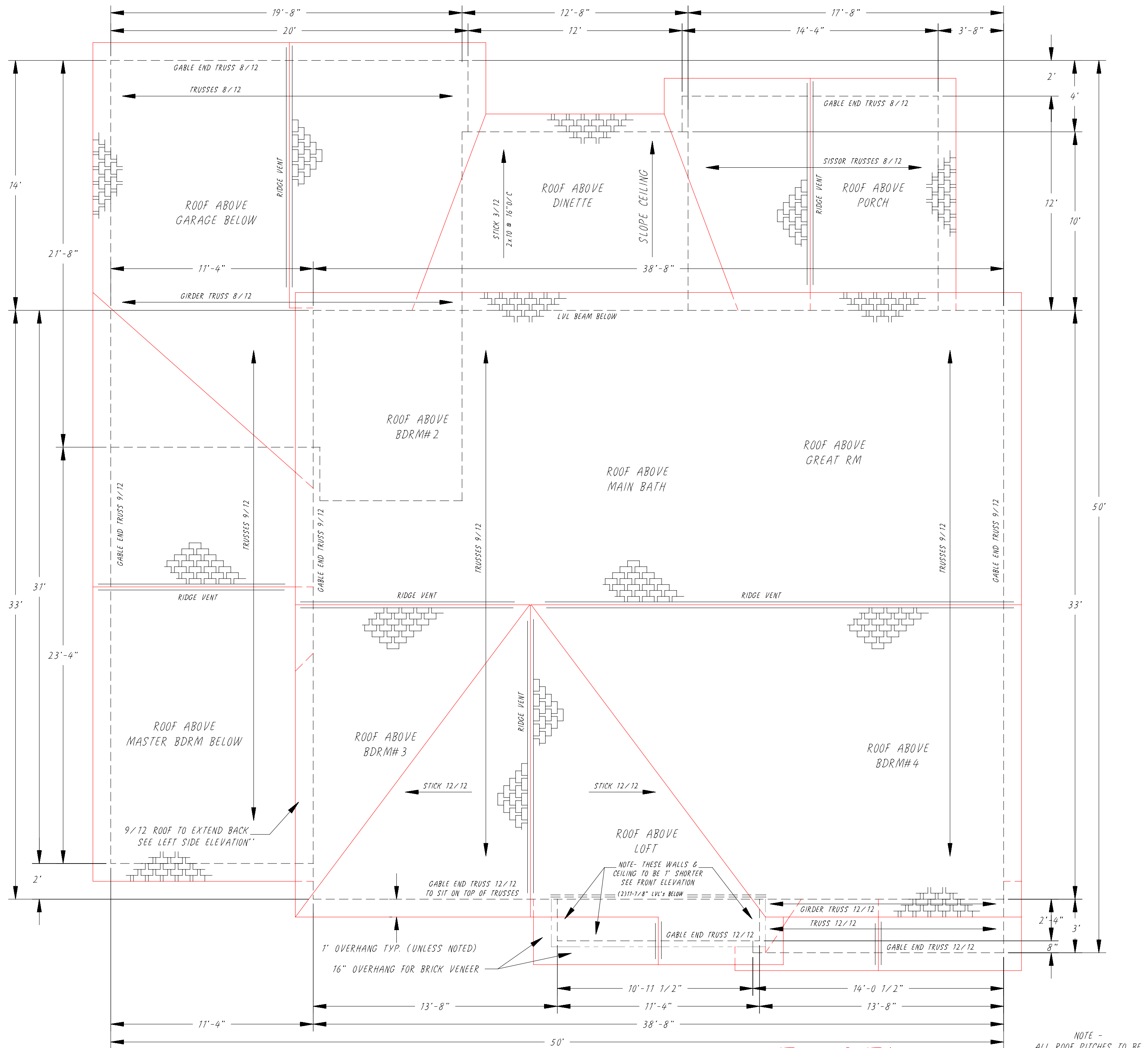
Roof Plan Front of House
