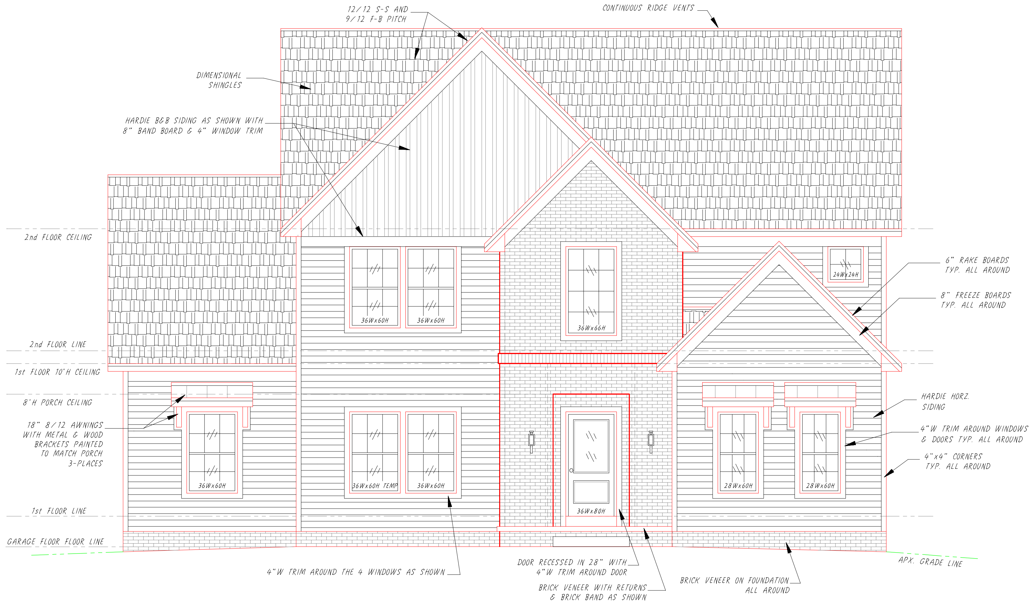
Front Elevation (S/L 10 - 5235 Preserve Lane)
