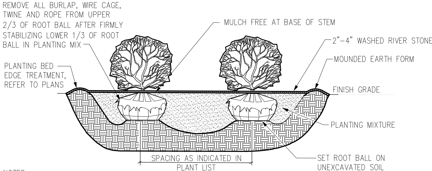
MASS SHRUB PLANTING DETAIL (B&B OR CONTAINER) NO SCALE
