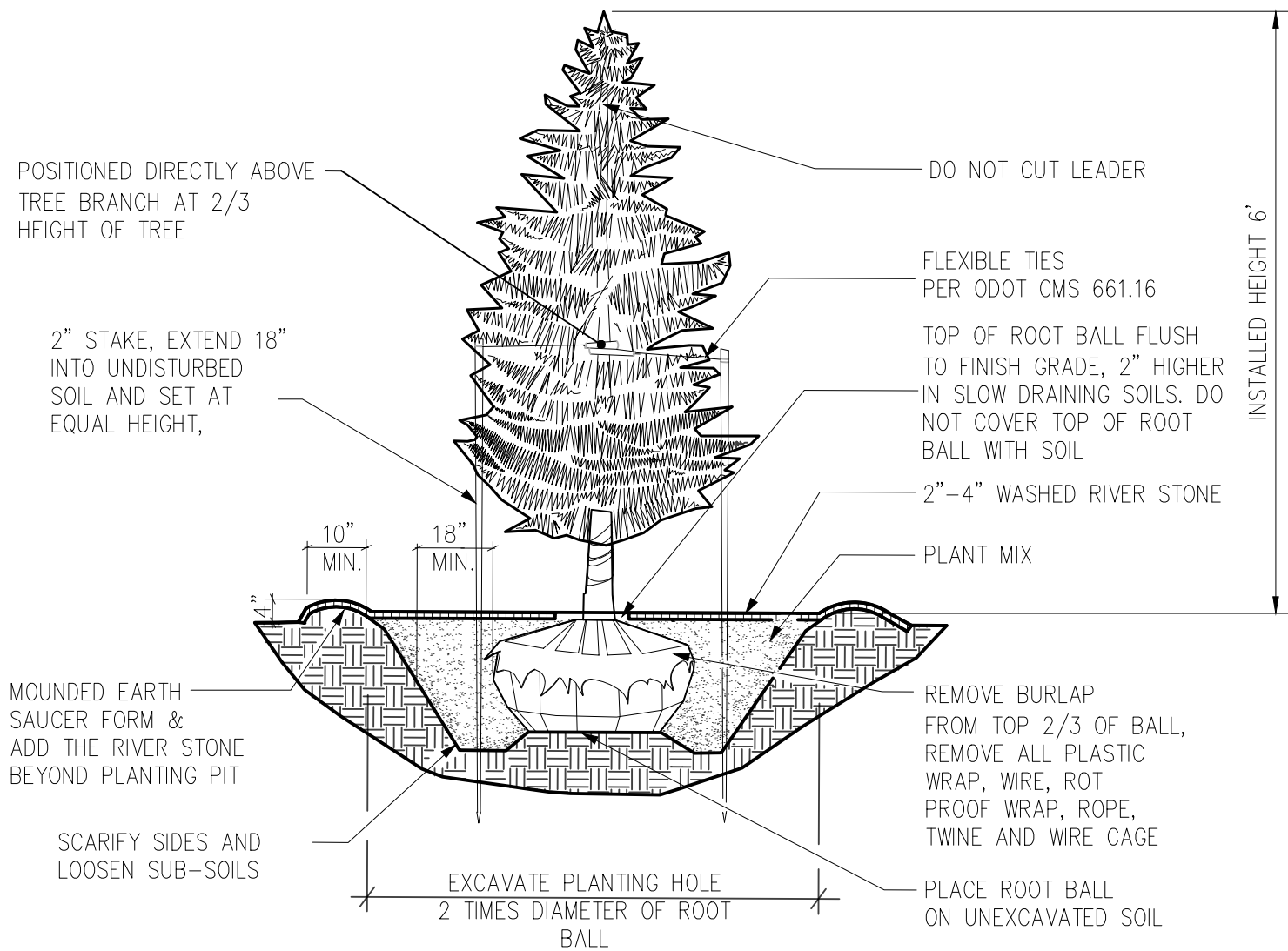
EVERGREEN TREE PLANTING DETAIL NO SCALE
