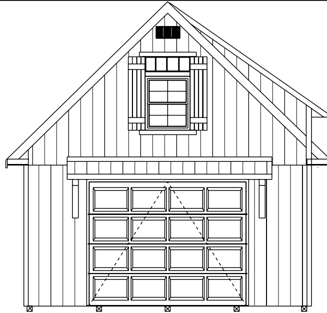
16X24 Front ELEVATION 30x36 window
