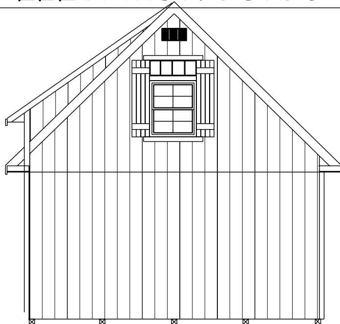
16X24 Rear ELEVATION 30X36
